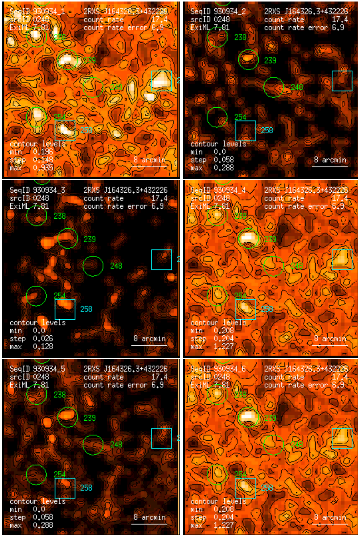
Figure 248: RASS 930934: detection 0248: band rate images, Gaussian filter: (1) PSPC channels 11 – 41, (2) 52 – 90, (3) 91 – 201, (4) 11 – 235, (5) 52 – 201, (6) 11 – 201. Broad band rates in counts/ks. Band rate contour levels in counts/ks/arcmin 2 .
