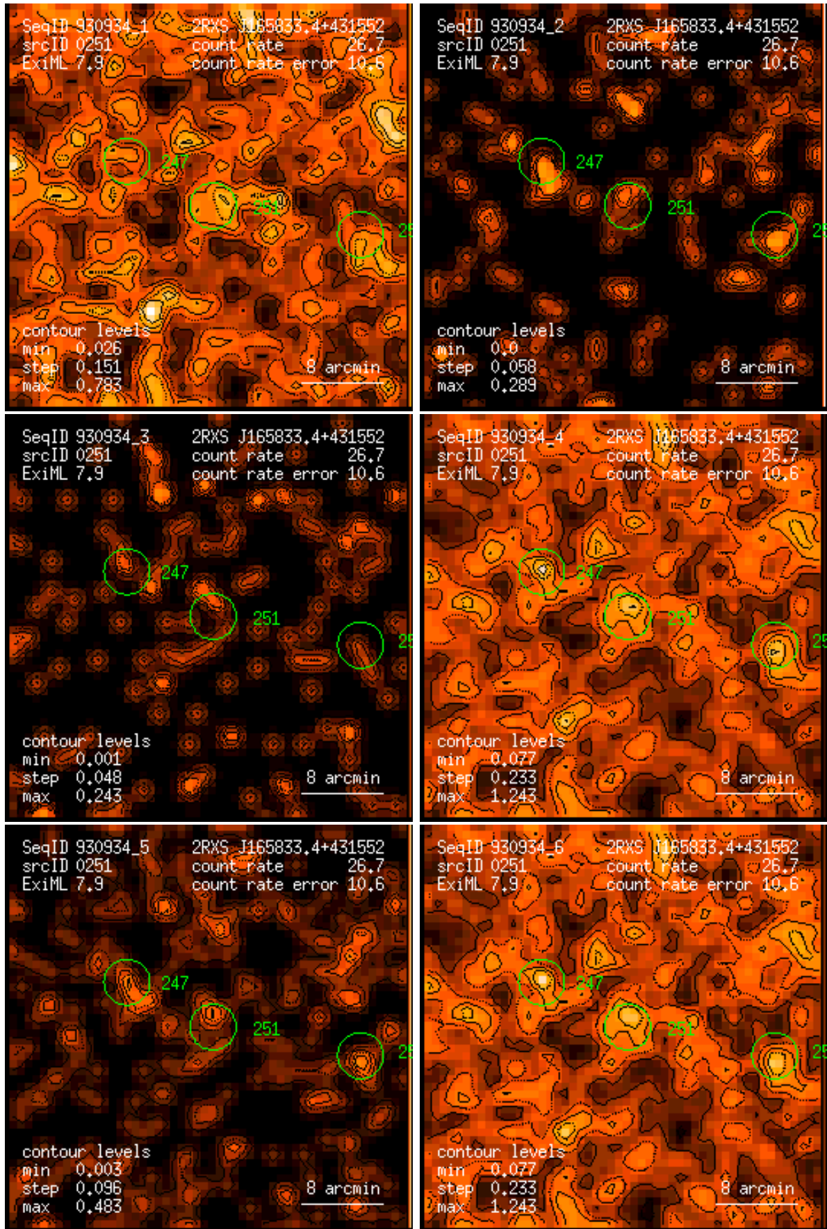
Figure 251: RASS 930934: detection 0251: band rate images, Gaussian filter: (1) PSPC channels 11 – 41, (2) 52 – 90, (3) 91 – 201, (4) 11 – 235, (5) 52 – 201, (6) 11 – 201. Broad band rates in counts/ks. Band rate contour levels in counts/ks/arcmin 2 .
