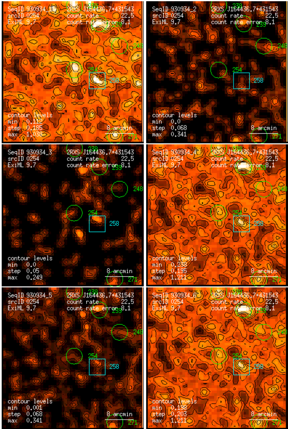
Figure 254: RASS 930934: detection 0254: band rate images, Gaussian filter: (1) PSPC channels 11 – 41, (2) 52 – 90, (3) 91 – 201, (4) 11 – 235, (5) 52 – 201, (6) 11 – 201. Broad band rates in counts/ks. Band rate contour levels in counts/ks/arcmin 2 .
