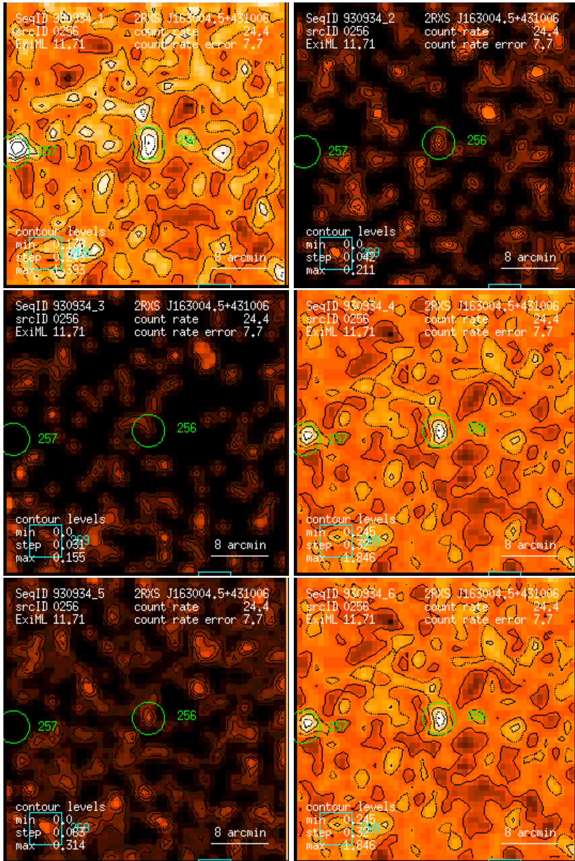
Figure 256: RASS 930934: detection 0256: band rate images, Gaussian filter: (1) PSPC channels 11 – 41, (2) 52 – 90, (3) 91 – 201, (4) 11 – 235, (5) 52 – 201, (6) 11 – 201. Broad band rates in counts/ks. Band rate contour levels in counts/ks/arcmin 2 .
