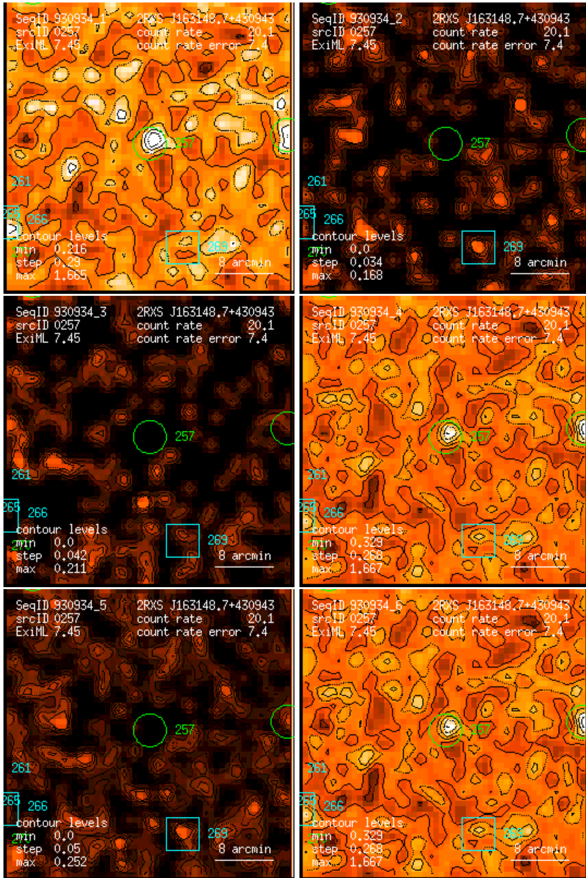
Figure 257: RASS 930934: detection 0257: band rate images, Gaussian filter: (1) PSPC channels 11 – 41, (2) 52 – 90, (3) 91 – 201, (4) 11 – 235, (5) 52 – 201, (6) 11 – 201. Broad band rates in counts/ks. Band rate contour levels in counts/ks/arcmin 2 .
