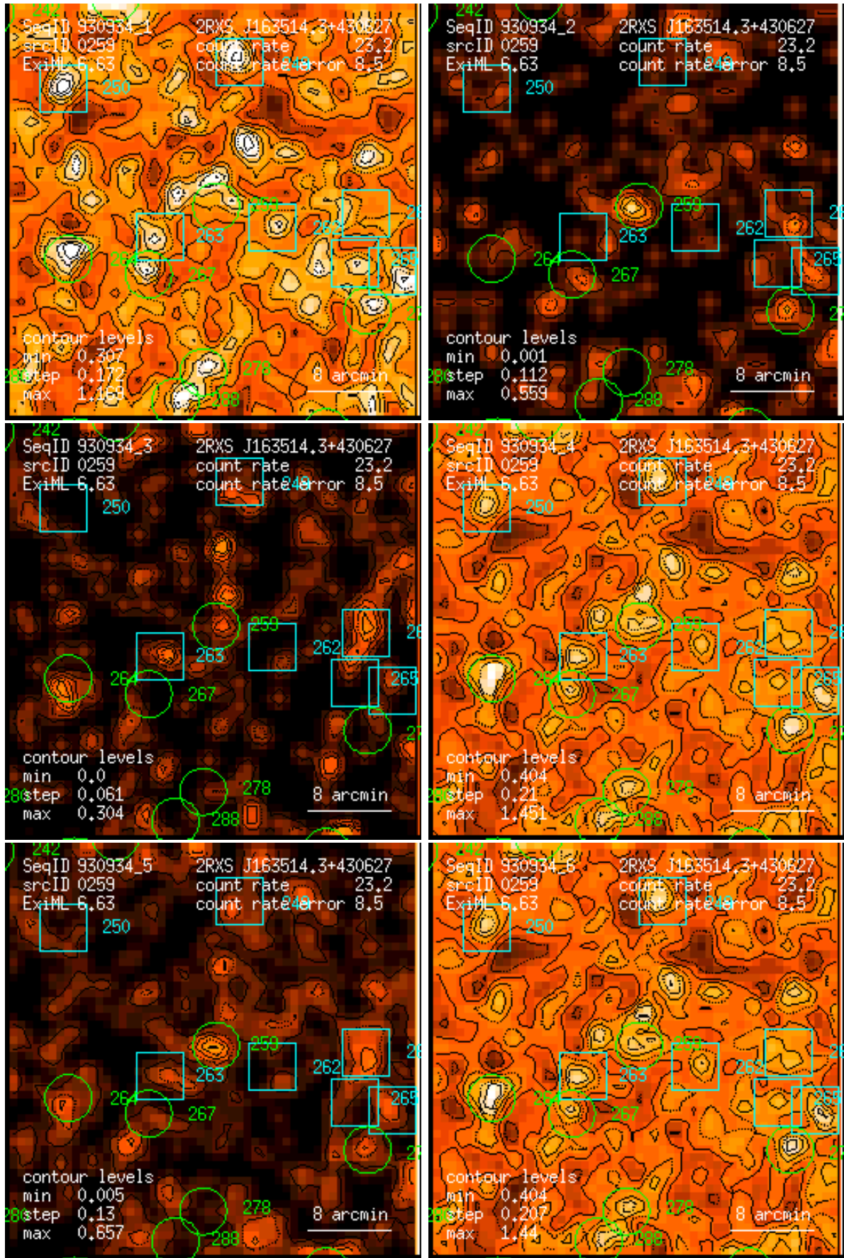
Figure 259: RASS 930934: detection 0259: band rate images, Gaussian filter: (1) PSPC channels 11 – 41, (2) 52 – 90, (3) 91 – 201, (4) 11 – 235, (5) 52 – 201, (6) 11 – 201. Broad band rates in counts/ks. Band rate contour levels in counts/ks/arcmin 2 .
