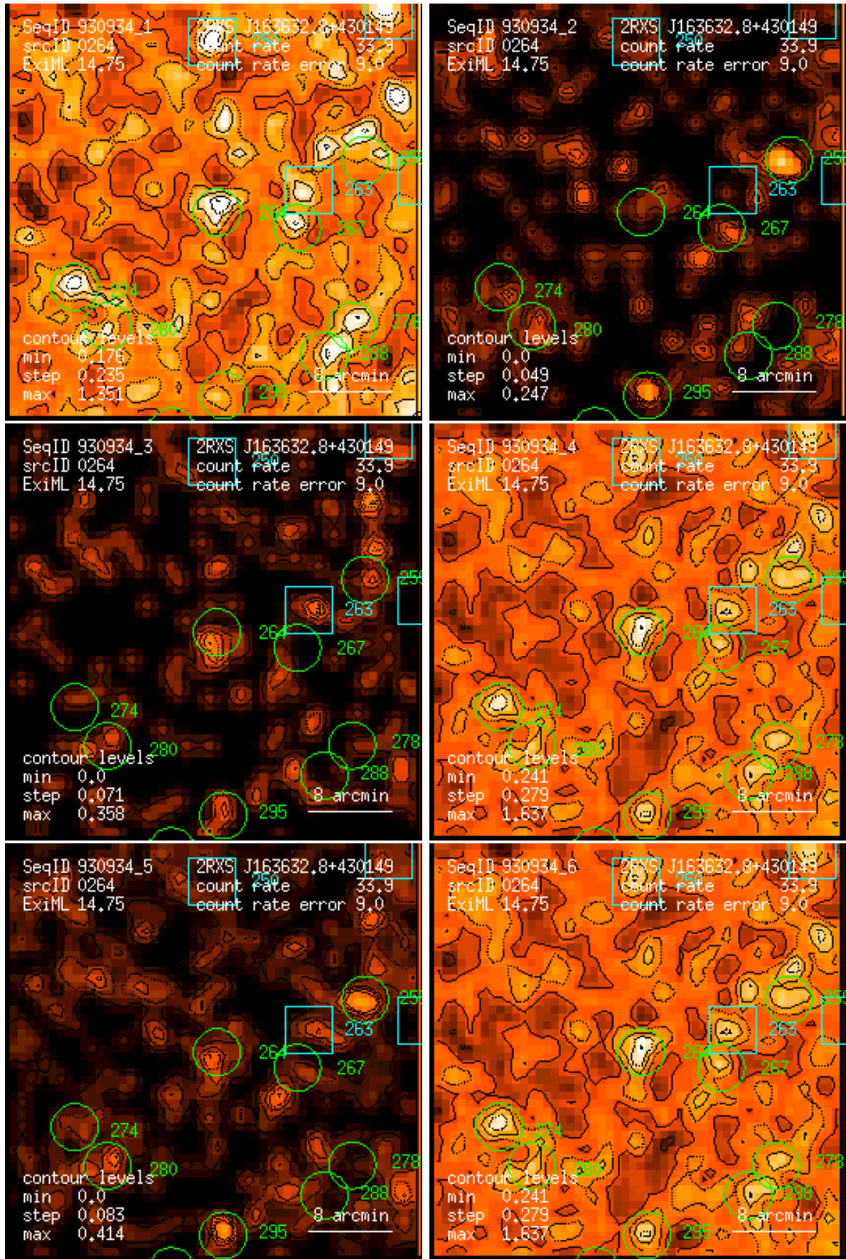
Figure 264: RASS 930934: detection 0264: band rate images, Gaussian filter: (1) PSPC channels 11 – 41, (2) 52 – 90, (3) 91 – 201, (4) 11 – 235, (5) 52 – 201, (6) 11 – 201. Broad band rates in counts/ks. Band rate contour levels in counts/ks/arcmin 2 .
