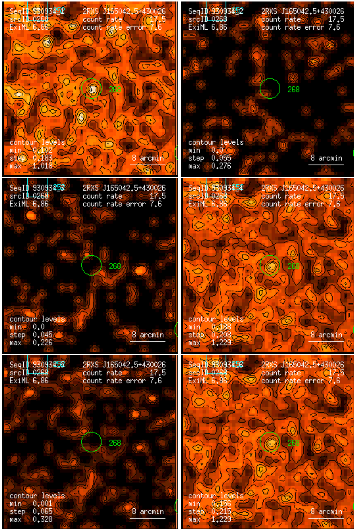
Figure 268: RASS 930934: detection 0268: band rate images, Gaussian filter: (1) PSPC channels 11 – 41, (2) 52 – 90, (3) 91 – 201, (4) 11 – 235, (5) 52 – 201, (6) 11 – 201. Broad band rates in counts/ks. Band rate contour levels in counts/ks/arcmin 2 .
