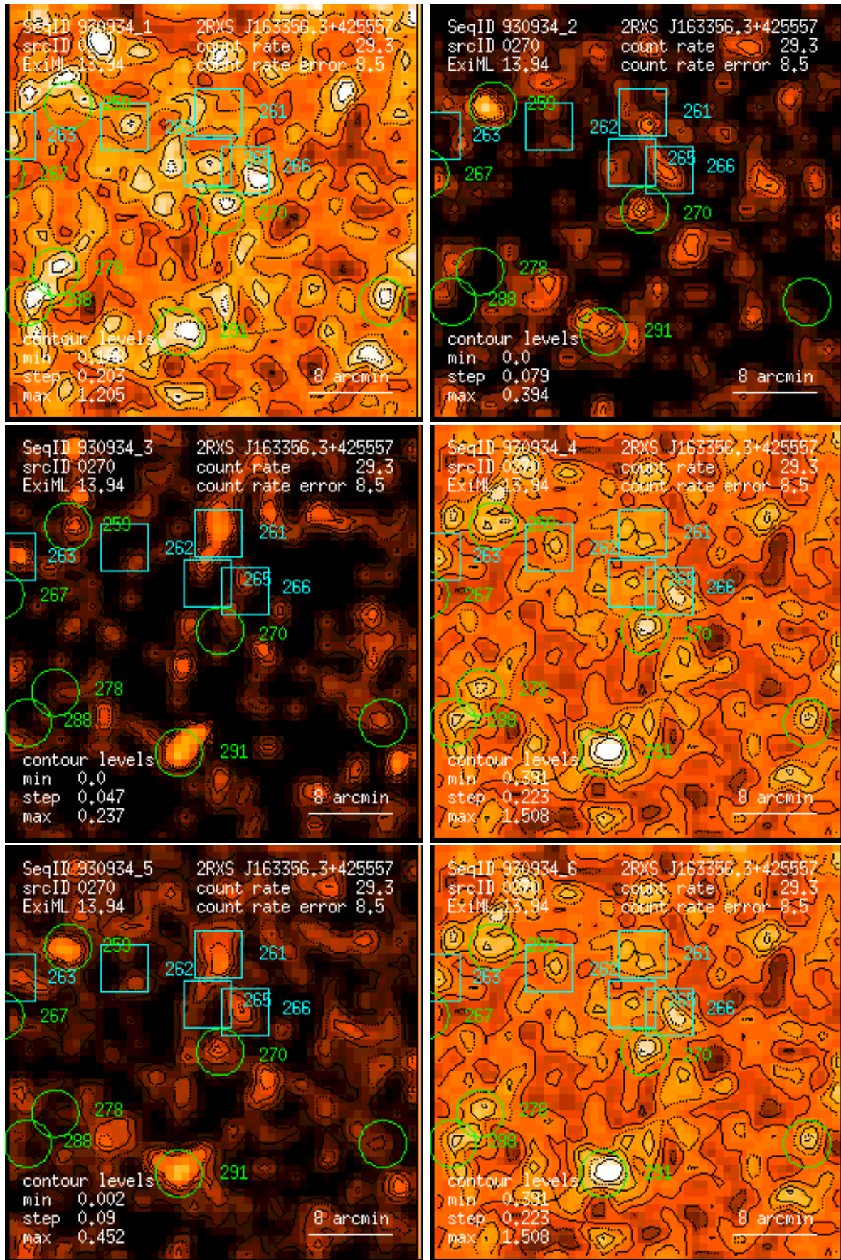
Figure 270: RASS 930934: detection 0270: band rate images, Gaussian filter: (1) PSPC channels 11 – 41, (2) 52 – 90, (3) 91 – 201, (4) 11 – 235, (5) 52 – 201, (6) 11 – 201. Broad band rates in counts/ks. Band rate contour levels in counts/ks/arcmin 2 .
