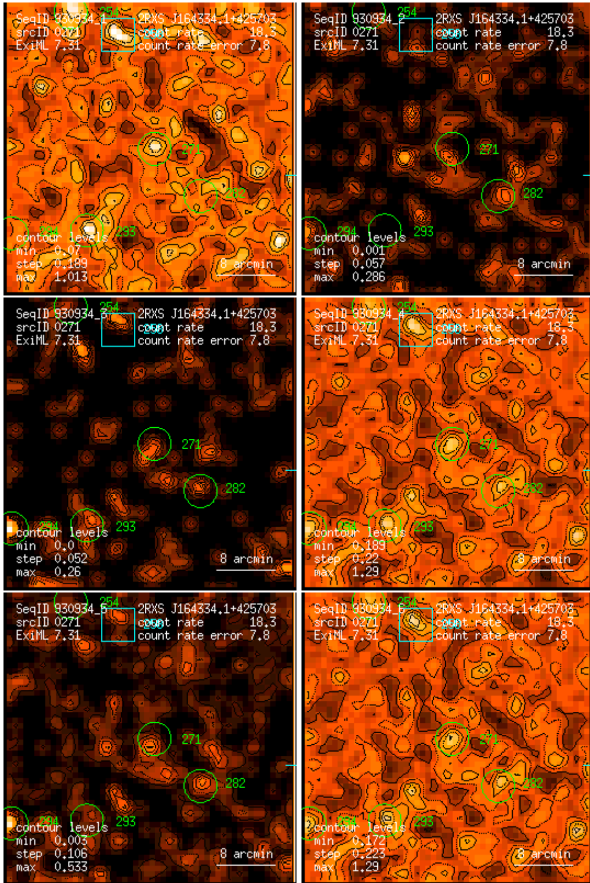
Figure 271: RASS 930934: detection 0271: band rate images, Gaussian filter: (1) PSPC channels 11 – 41, (2) 52 – 90, (3) 91 – 201, (4) 11 – 235, (5) 52 – 201, (6) 11 – 201. Broad band rates in counts/ks. Band rate contour levels in counts/ks/arcmin 2 .
