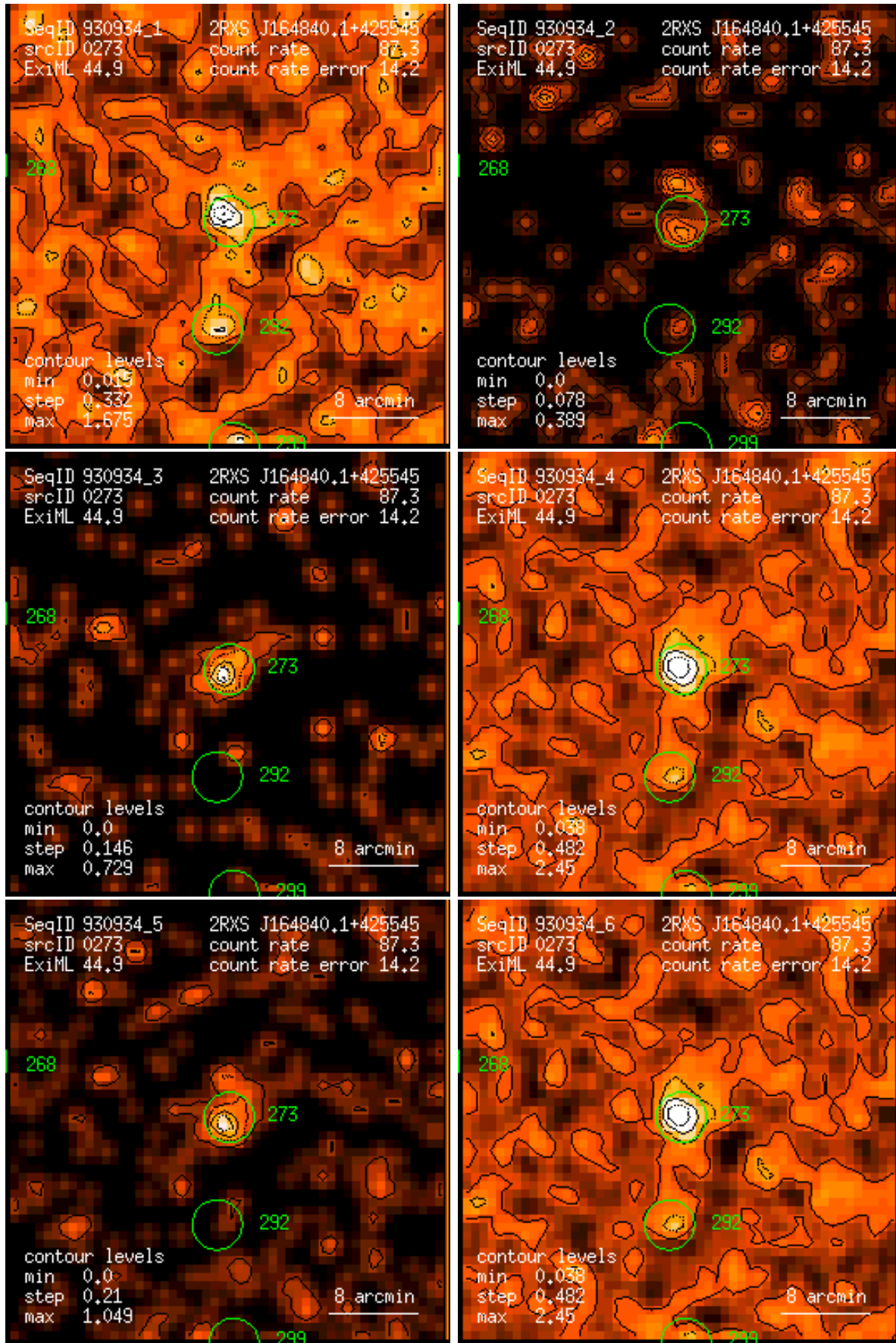
Figure 273: RASS 930934: detection 0273: band rate images, Gaussian filter: (1) PSPC channels 11 – 41, (2) 52 – 90, (3) 91 – 201, (4) 11 – 235, (5) 52 – 201, (6) 11 – 201. Broad band rates in counts/ks. Band rate contour levels in counts/ks/arcmin 2 .
