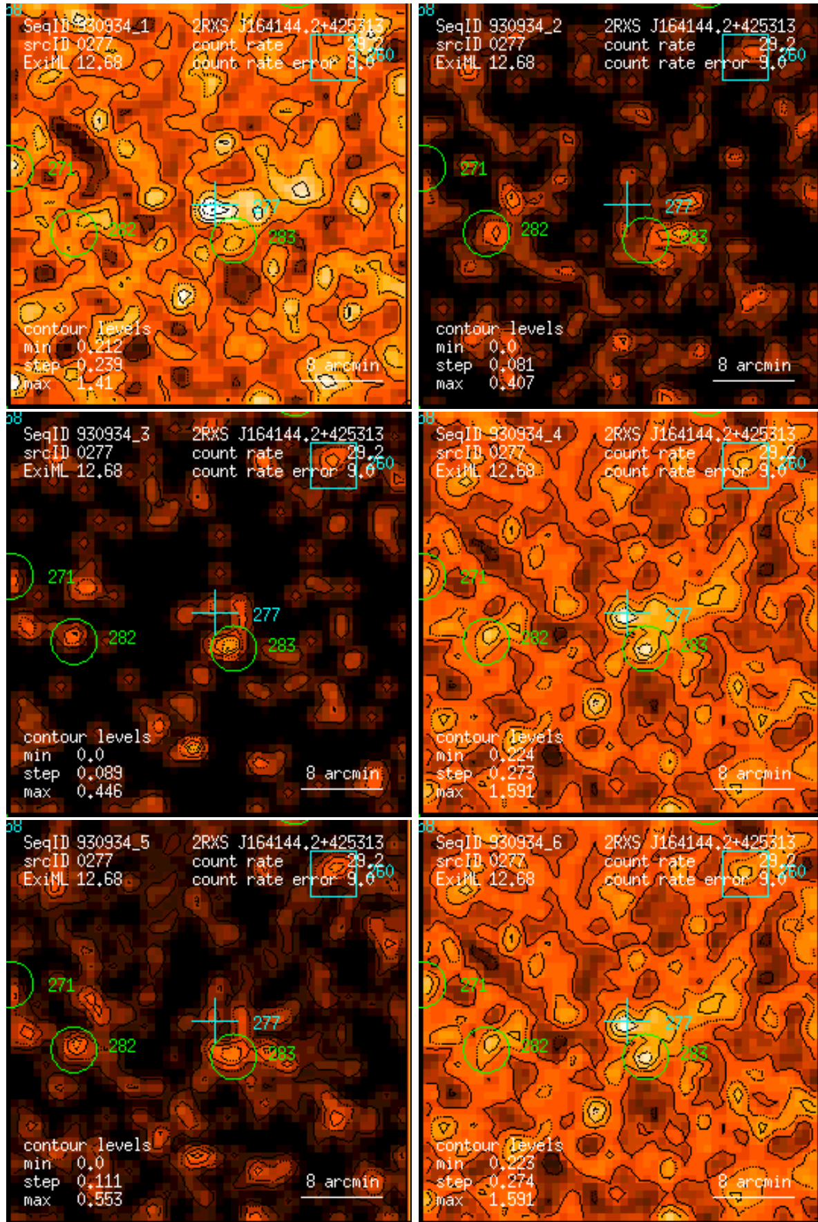
Figure 277: RASS 930934: detection 0277: band rate images, Gaussian filter: (1) PSPC channels 11 – 41, (2) 52 – 90, (3) 91 – 201, (4) 11 – 235, (5) 52 – 201, (6) 11 – 201. Broad band rates in counts/ks. Band rate contour levels in counts/ks/arcmin 2 .
