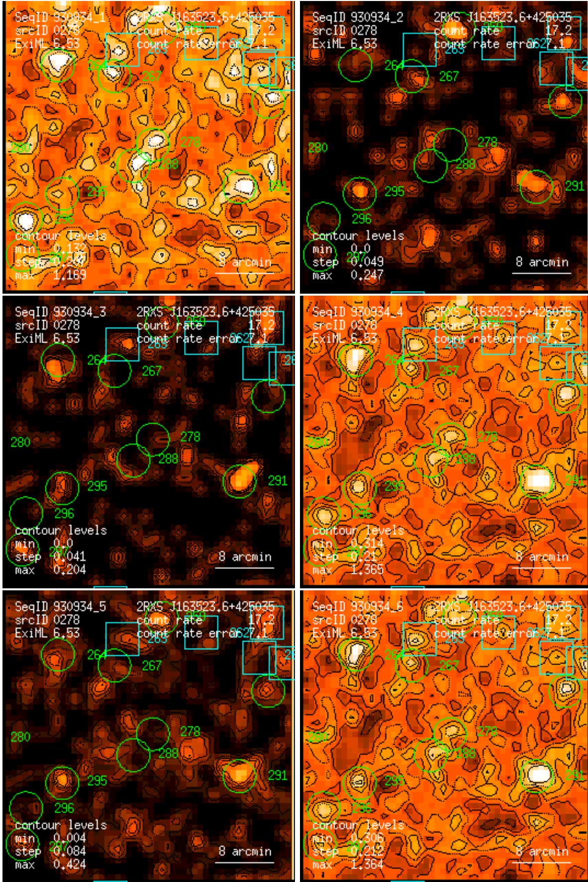
Figure 278: RASS 930934: detection 0278: band rate images, Gaussian filter: (1) PSPC channels 11 – 41, (2) 52 – 90, (3) 91 – 201, (4) 11 – 235, (5) 52 – 201, (6) 11 – 201. Broad band rates in counts/ks. Band rate contour levels in counts/ks/arcmin 2 .
