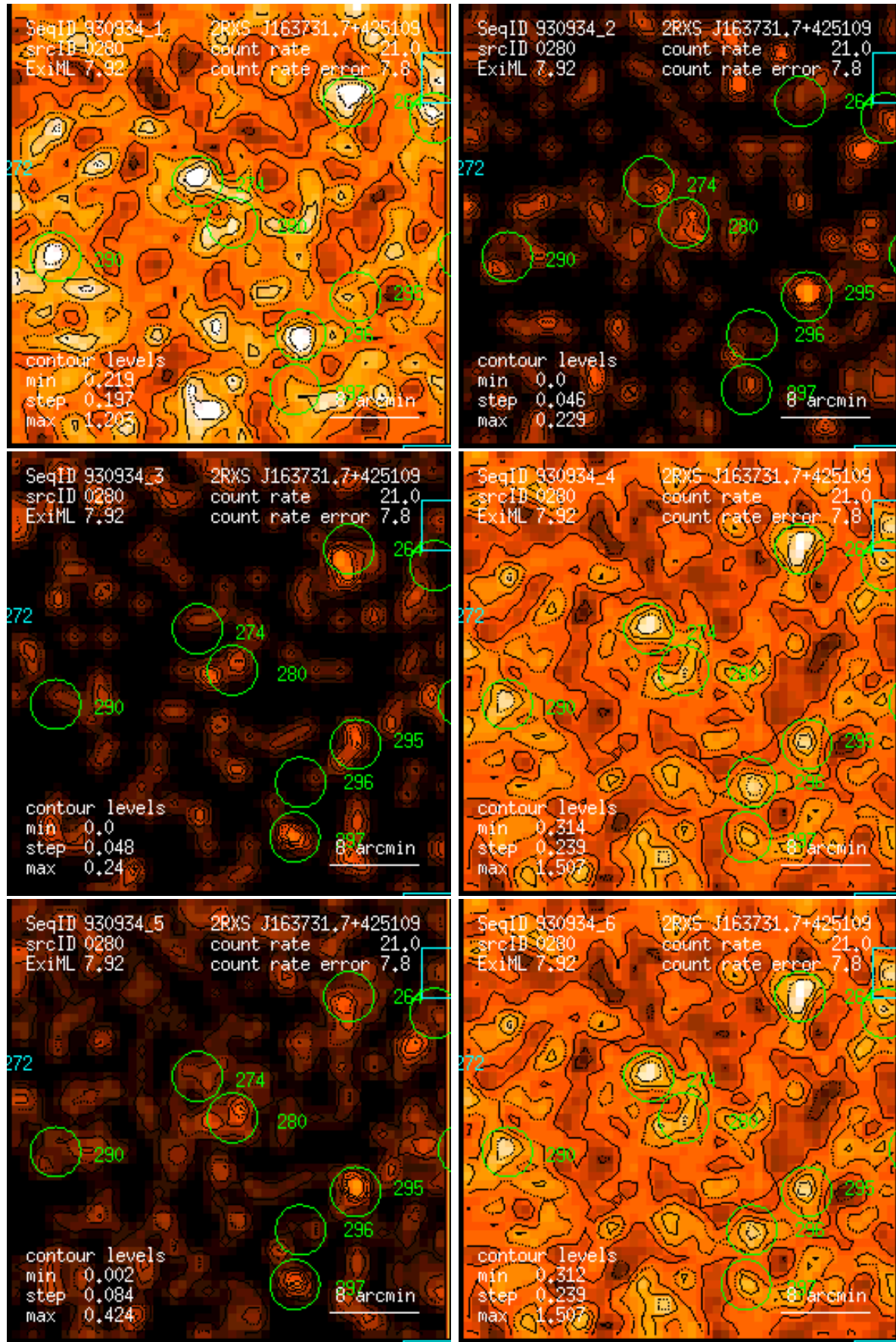
Figure 280: RASS 930934: detection 0280: band rate images, Gaussian filter: (1) PSPC channels 11 – 41, (2) 52 – 90, (3) 91 – 201, (4) 11 – 235, (5) 52 – 201, (6) 11 – 201. Broad band rates in counts/ks. Band rate contour levels in counts/ks/arcmin 2 .
