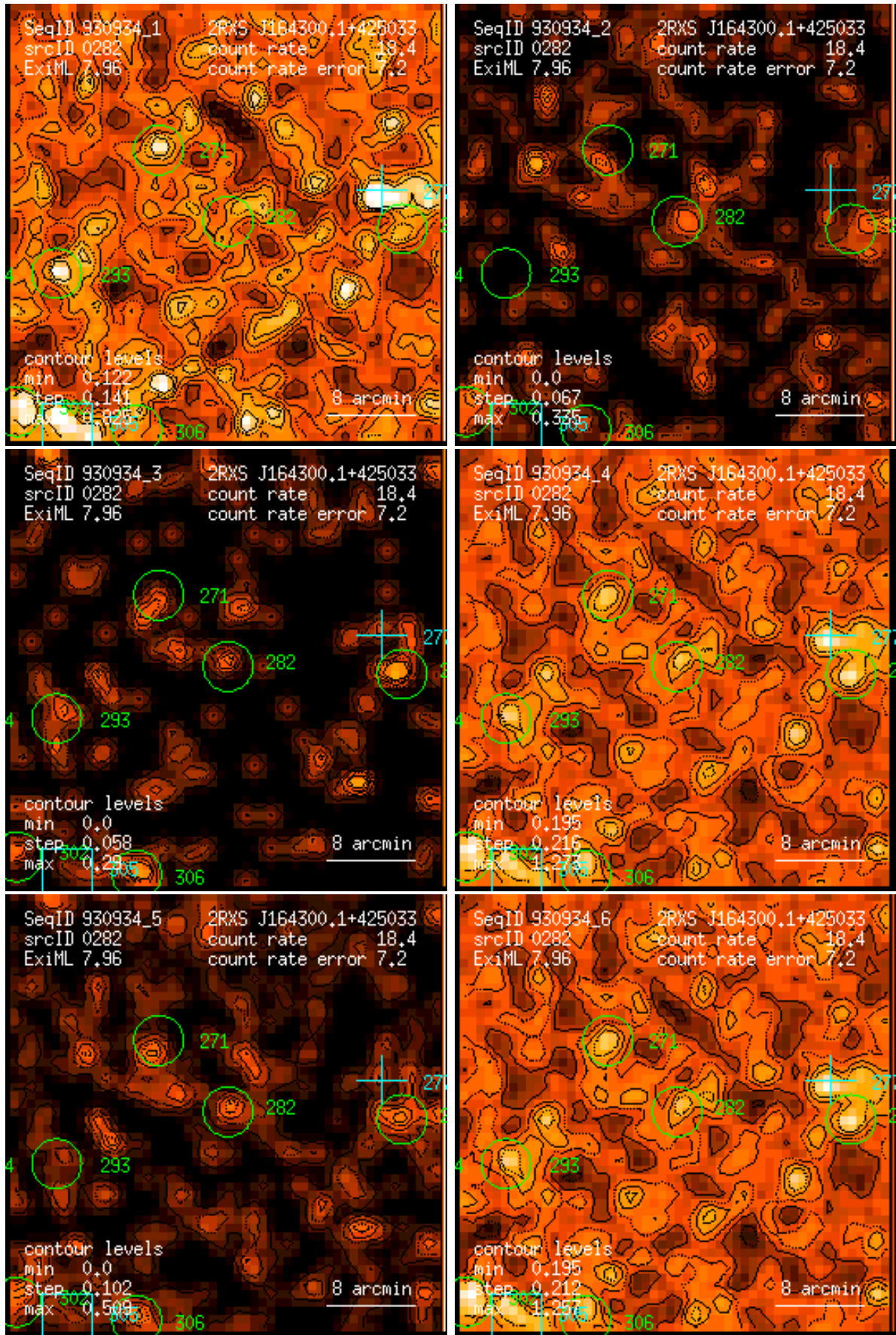
Figure 282: RASS 930934: detection 0282: band rate images, Gaussian filter: (1) PSPC channels 11 – 41, (2) 52 – 90, (3) 91 – 201, (4) 11 – 235, (5) 52 – 201, (6) 11 – 201. Broad band rates in counts/ks. Band rate contour levels in counts/ks/arcmin 2 .
