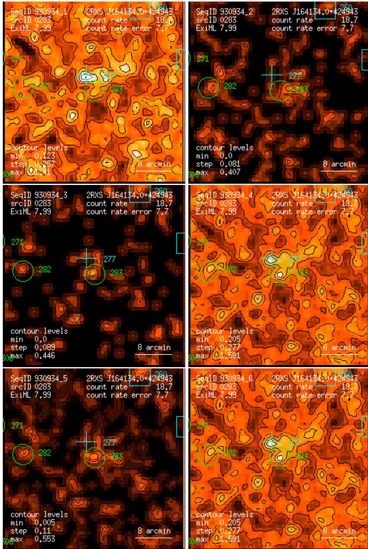
Figure 283: RASS 930934: detection 0283: band rate images, Gaussian filter: (1) PSPC channels 11 – 41, (2) 52 – 90, (3) 91 – 201, (4) 11 – 235, (5) 52 – 201, (6) 11 – 201. Broad band rates in counts/ks. Band rate contour levels in counts/ks/arcmin 2 .
