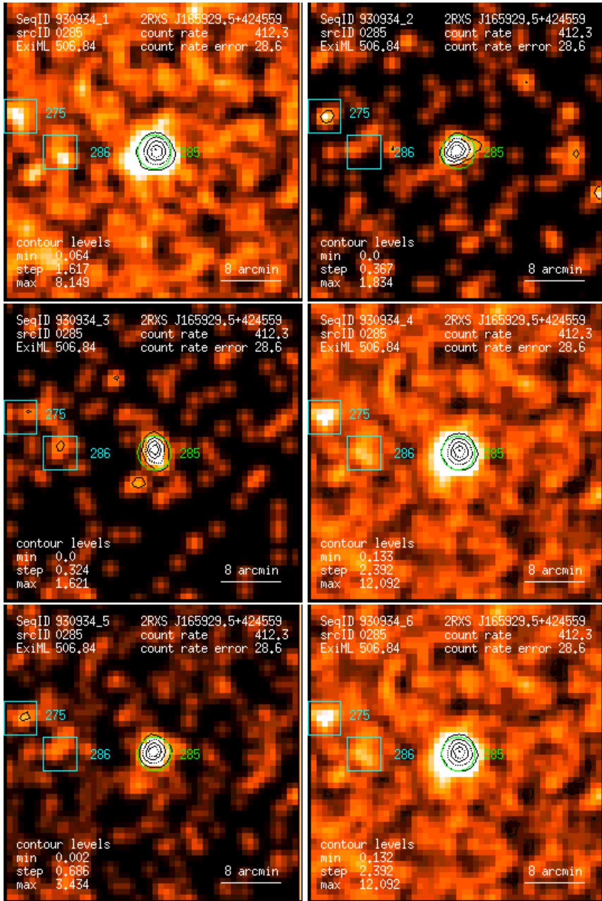
Figure 285: RASS 930934: detection 0285: band rate images, Gaussian filter: (1) PSPC channels 11 – 41, (2) 52 – 90, (3) 91 – 201, (4) 11 – 235, (5) 52 – 201, (6) 11 – 201. Broad band rates in counts/ks. Band rate contour levels in counts/ks/arcmin 2 .
