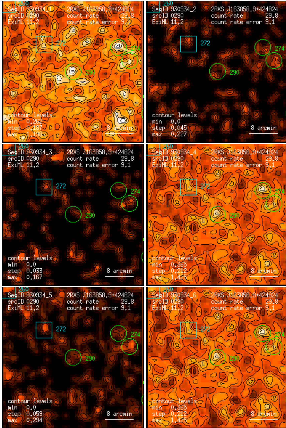
Figure 290: RASS 930934: detection 0290: band rate images, Gaussian filter: (1) PSPC channels 11 – 41, (2) 52 – 90, (3) 91 – 201, (4) 11 – 235, (5) 52 – 201, (6) 11 – 201. Broad band rates in counts/ks. Band rate contour levels in counts/ks/arcmin 2 .
