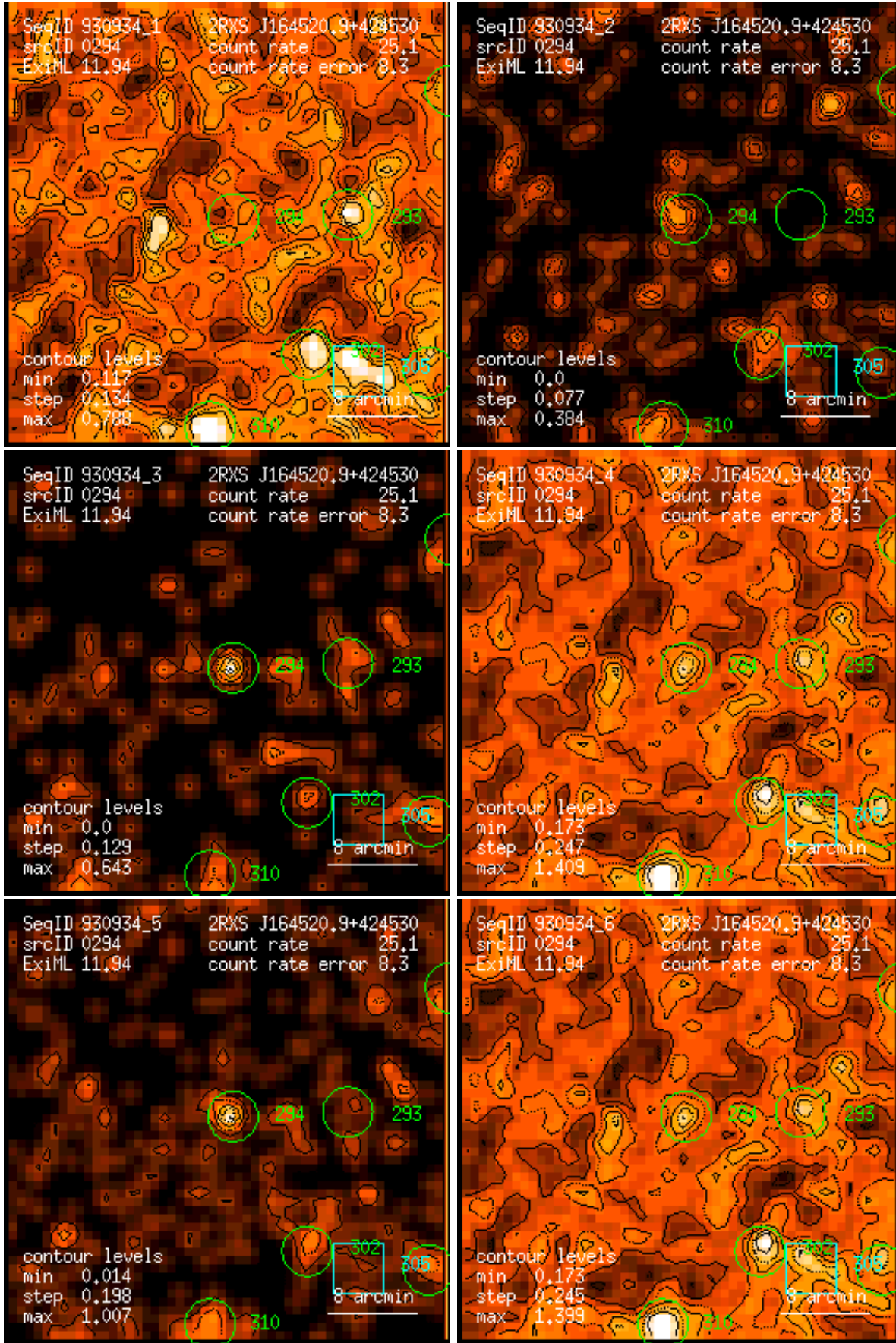
Figure 294: RASS 930934: detection 0294: band rate images, Gaussian filter: (1) PSPC channels 11 – 41, (2) 52 – 90, (3) 91 – 201, (4) 11 – 235, (5) 52 – 201, (6) 11 – 201. Broad band rates in counts/ks. Band rate contour levels in counts/ks/arcmin 2 .
