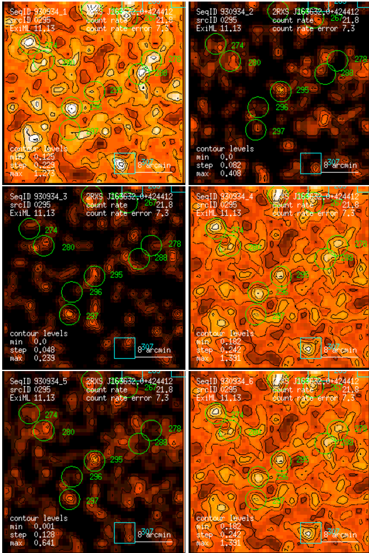
Figure 295: RASS 930934: detection 0295: band rate images, Gaussian filter: (1) PSPC channels 11 – 41, (2) 52 – 90, (3) 91 – 201, (4) 11 – 235, (5) 52 – 201, (6) 11 – 201. Broad band rates in counts/ks. Band rate contour levels in counts/ks/arcmin 2 .
