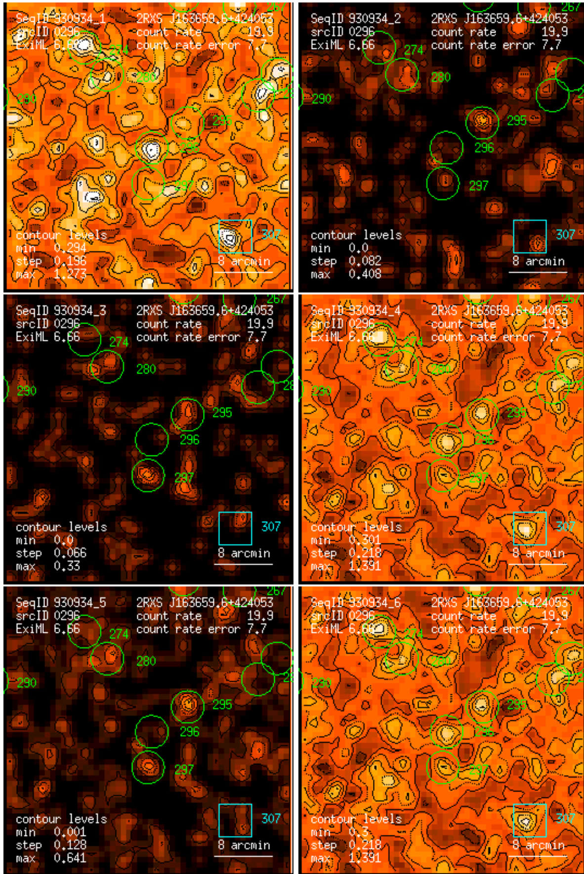
Figure 296: RASS 930934: detection 0296: band rate images, Gaussian filter: (1) PSPC channels 11 – 41, (2) 52 – 90, (3) 91 – 201, (4) 11 – 235, (5) 52 – 201, (6) 11 – 201. Broad band rates in counts/ks. Band rate contour levels in counts/ks/arcmin 2 .
