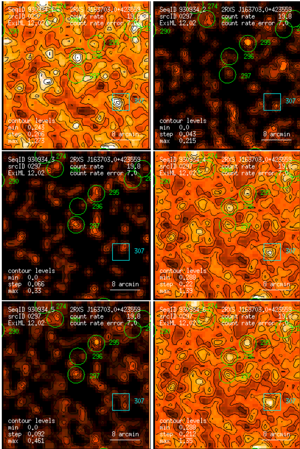
Figure 297: RASS 930934: detection 0297: band rate images, Gaussian filter: (1) PSPC channels 11 – 41, (2) 52 – 90, (3) 91 – 201, (4) 11 – 235, (5) 52 – 201, (6) 11 – 201. Broad band rates in counts/ks. Band rate contour levels in counts/ks/arcmin 2 .
