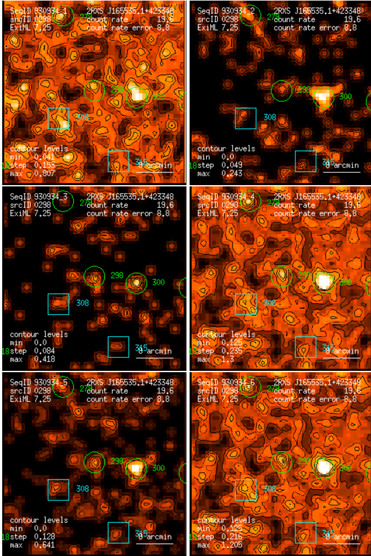
Figure 298: RASS 930934: detection 0298: band rate images, Gaussian filter: (1) PSPC channels 11 – 41, (2) 52 – 90, (3) 91 – 201, (4) 11 – 235, (5) 52 – 201, (6) 11 – 201. Broad band rates in counts/ks. Band rate contour levels in counts/ks/arcmin 2 .
