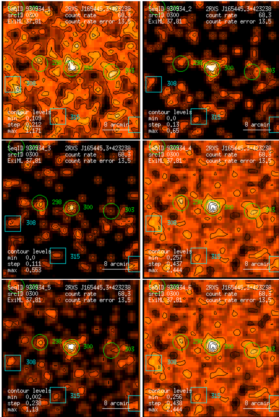
Figure 300: RASS 930934: detection 0300: band rate images, Gaussian filter: (1) PSPC channels 11 – 41, (2) 52 – 90, (3) 91 – 201, (4) 11 – 235, (5) 52 – 201, (6) 11 – 201. Broad band rates in counts/ks. Band rate contour levels in counts/ks/arcmin 2 .
