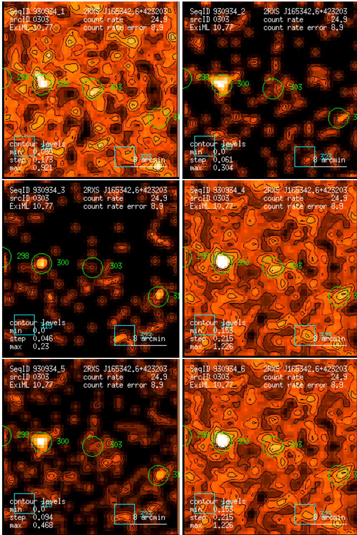
Figure 303: RASS 930934: detection 0303: band rate images, Gaussian filter: (1) PSPC channels 11 – 41, (2) 52 – 90, (3) 91 – 201, (4) 11 – 235, (5) 52 – 201, (6) 11 – 201. Broad band rates in counts/ks. Band rate contour levels in counts/ks/arcmin 2 .
