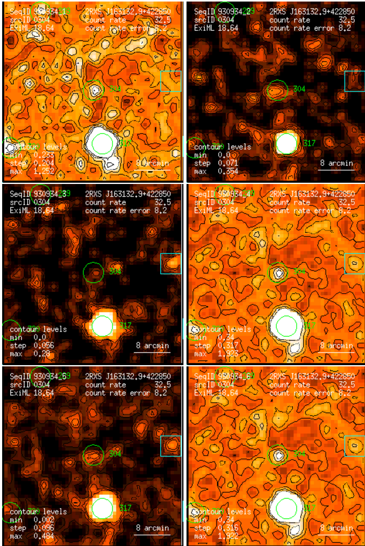
Figure 304: RASS 930934: detection 0304: band rate images, Gaussian filter: (1) PSPC channels 11 – 41, (2) 52 – 90, (3) 91 – 201, (4) 11 – 235, (5) 52 – 201, (6) 11 – 201. Broad band rates in counts/ks. Band rate contour levels in counts/ks/arcmin 2 .
