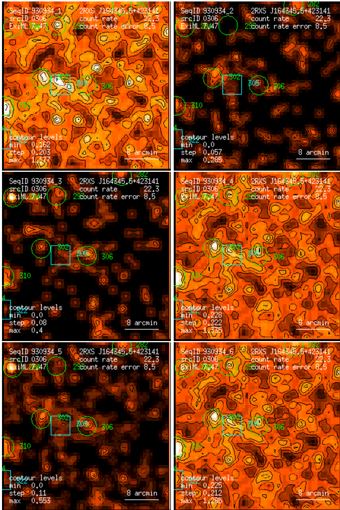
Figure 306: RASS 930934: detection 0306: band rate images, Gaussian filter: (1) PSPC channels 11 – 41, (2) 52 – 90, (3) 91 – 201, (4) 11 – 235, (5) 52 – 201, (6) 11 – 201. Broad band rates in counts/ks. Band rate contour levels in counts/ks/arcmin 2 .
