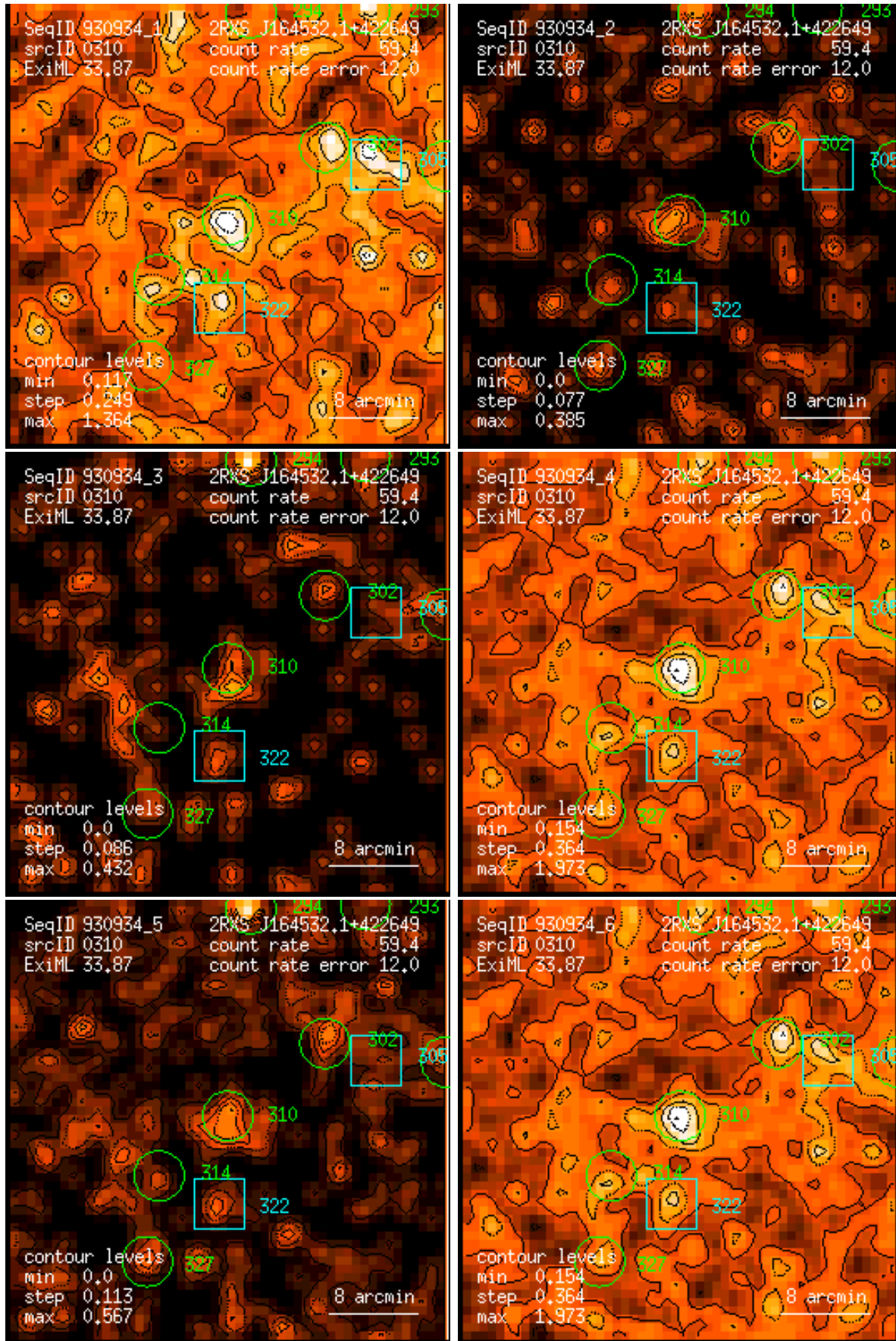
Figure 310: RASS 930934: detection 0310: band rate images, Gaussian filter: (1) PSPC channels 11 – 41, (2) 52 – 90, (3) 91 – 201, (4) 11 – 235, (5) 52 – 201, (6) 11 – 201. Broad band rates in counts/ks. Band rate contour levels in counts/ks/arcmin 2 .
