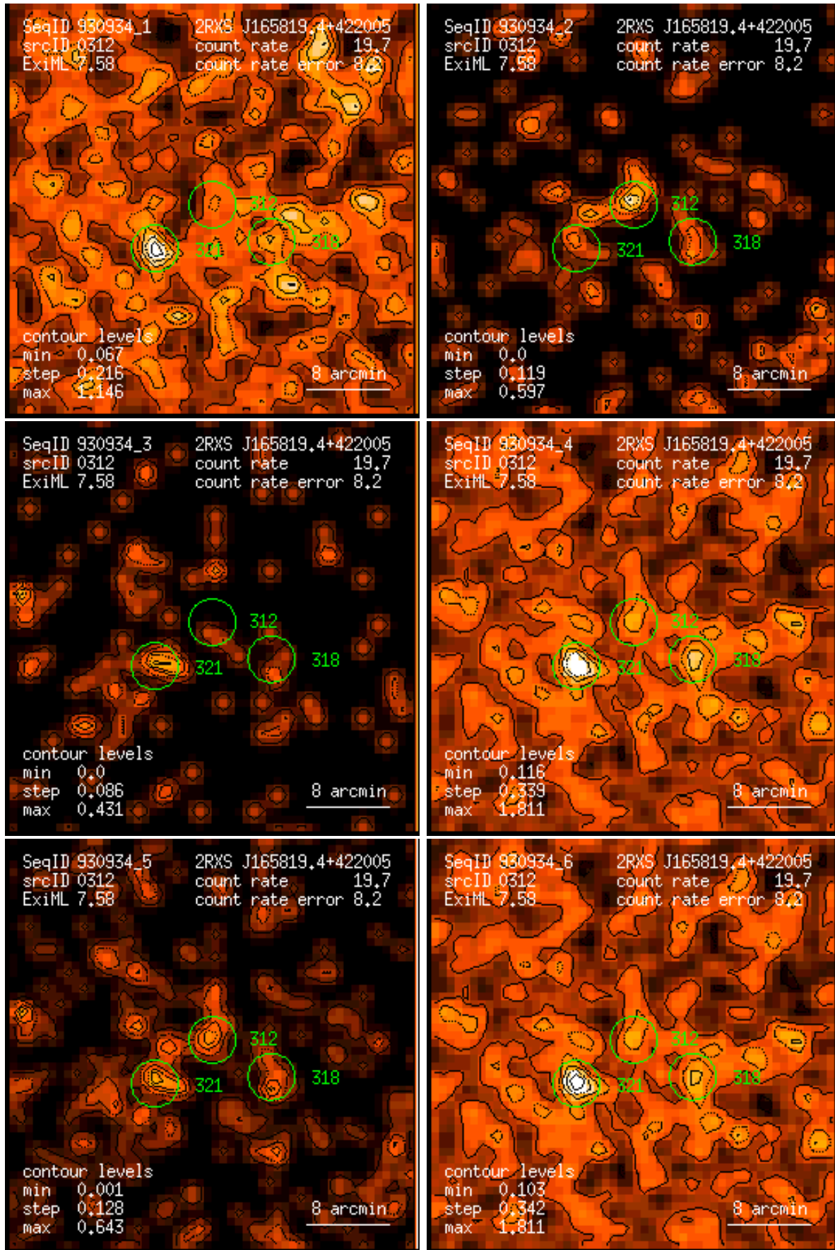
Figure 312: RASS 930934: detection 0312: band rate images, Gaussian filter: (1) PSPC channels 11 – 41, (2) 52 – 90, (3) 91 – 201, (4) 11 – 235, (5) 52 – 201, (6) 11 – 201. Broad band rates in counts/ks. Band rate contour levels in counts/ks/arcmin 2 .
