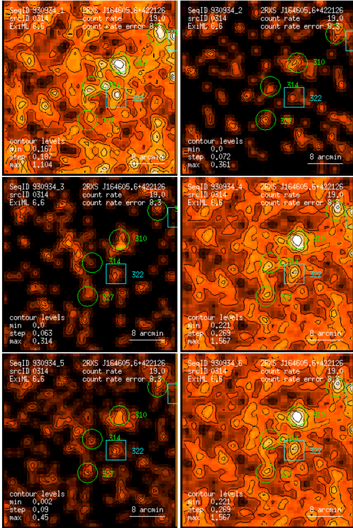
Figure 314: RASS 930934: detection 0314: band rate images, Gaussian filter: (1) PSPC channels 11 – 41, (2) 52 – 90, (3) 91 – 201, (4) 11 – 235, (5) 52 – 201, (6) 11 – 201. Broad band rates in counts/ks. Band rate contour levels in counts/ks/arcmin 2 .
