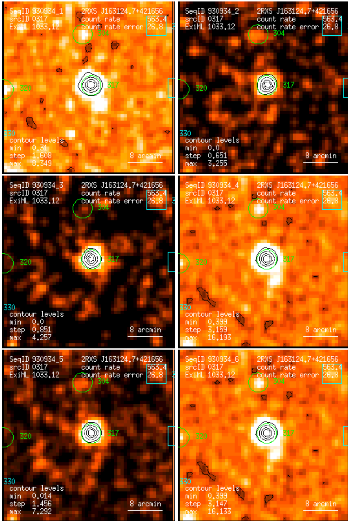
Figure 317: RASS 930934: detection 0317: band rate images, Gaussian filter: (1) PSPC channels 11 – 41, (2) 52 – 90, (3) 91 – 201, (4) 11 – 235, (5) 52 – 201, (6) 11 – 201. Broad band rates in counts/ks. Band rate contour levels in counts/ks/arcmin 2 .
