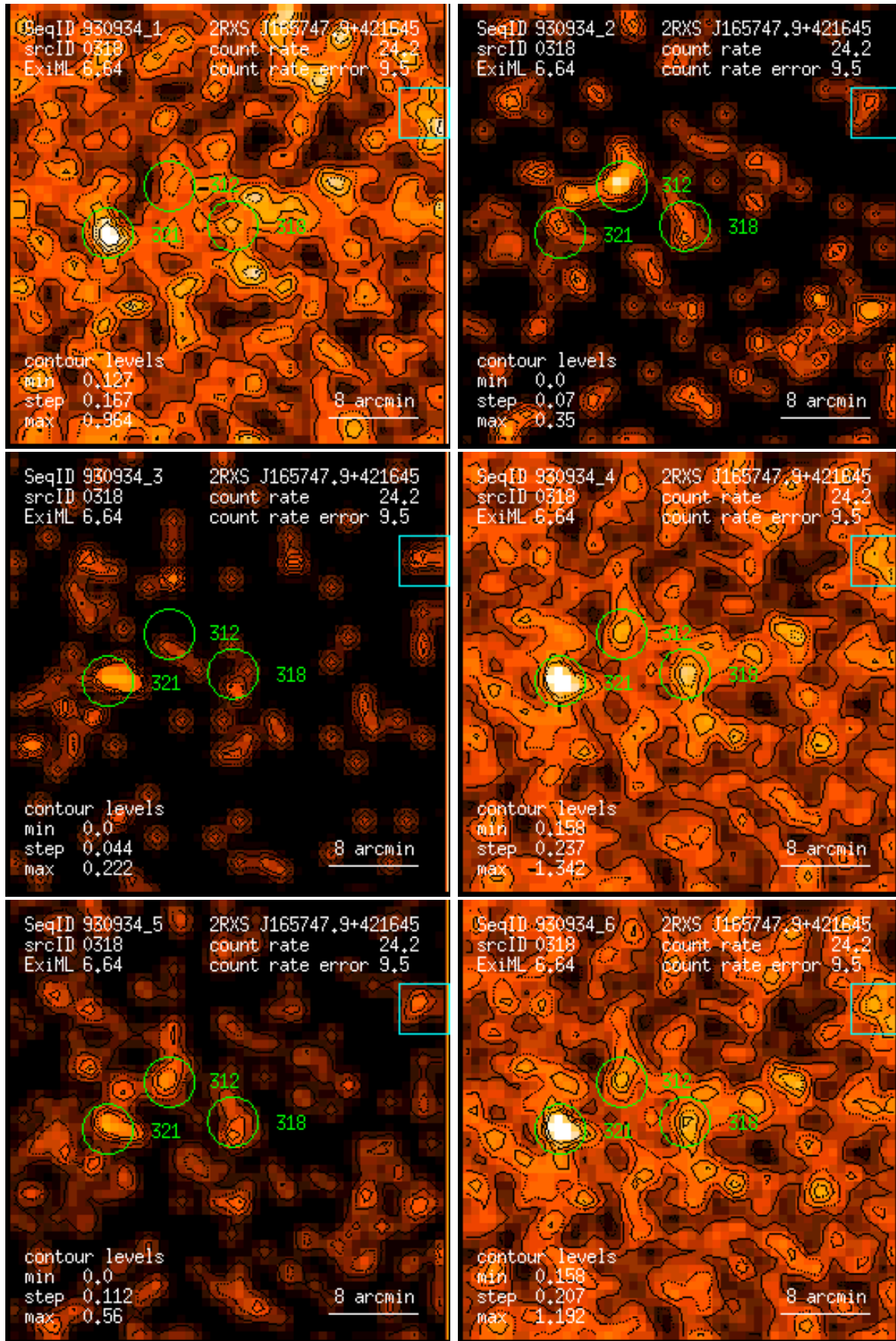
Figure 318: RASS 930934: detection 0318: band rate images, Gaussian filter: (1) PSPC channels 11 – 41, (2) 52 – 90, (3) 91 – 201, (4) 11 – 235, (5) 52 – 201, (6) 11 – 201. Broad band rates in counts/ks. Band rate contour levels in counts/ks/arcmin 2 .
