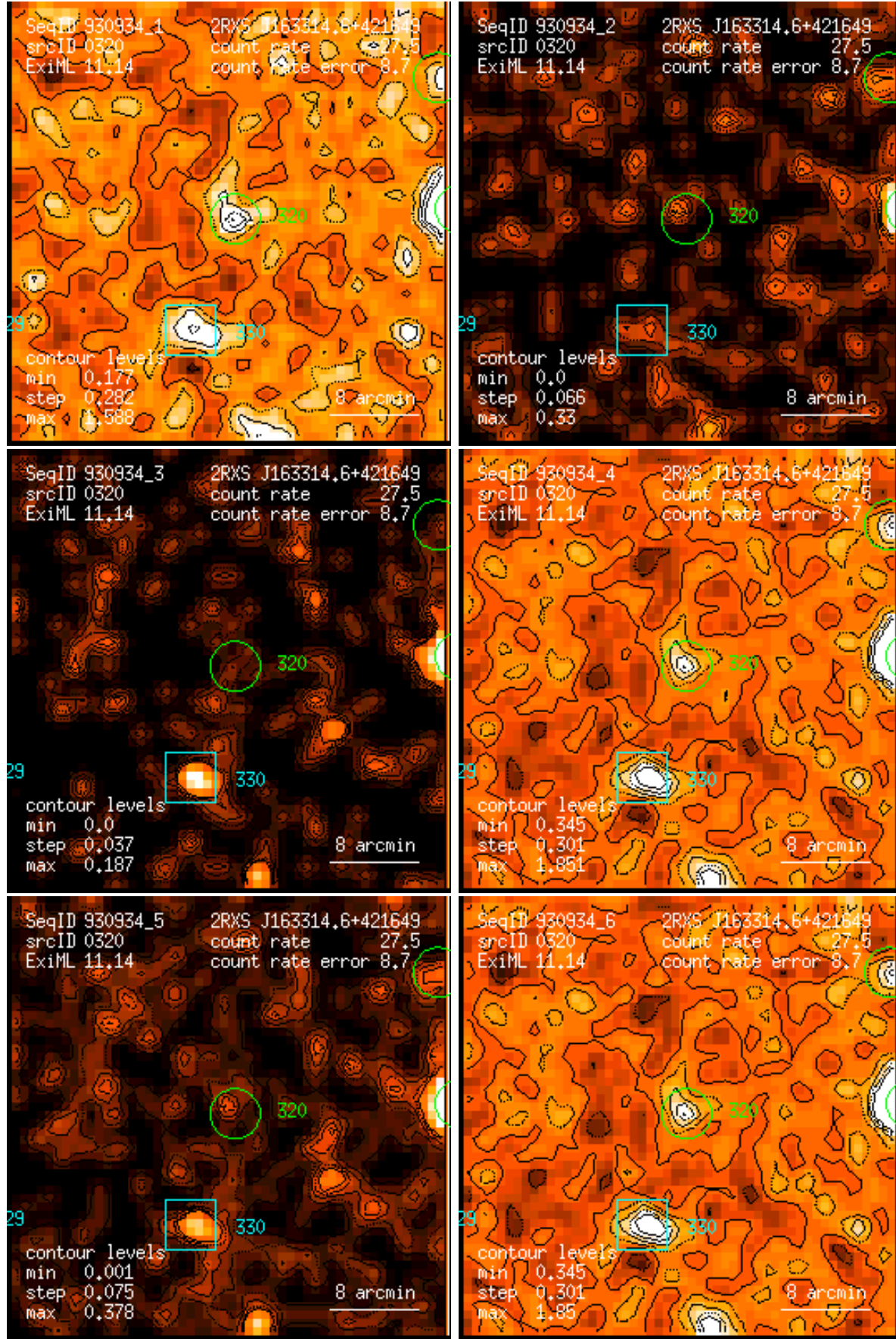
Figure 320: RASS 930934: detection 0320: band rate images, Gaussian filter: (1) PSPC channels 11 – 41, (2) 52 – 90, (3) 91 – 201, (4) 11 – 235, (5) 52 – 201, (6) 11 – 201. Broad band rates in counts/ks. Band rate contour levels in counts/ks/arcmin 2 .
