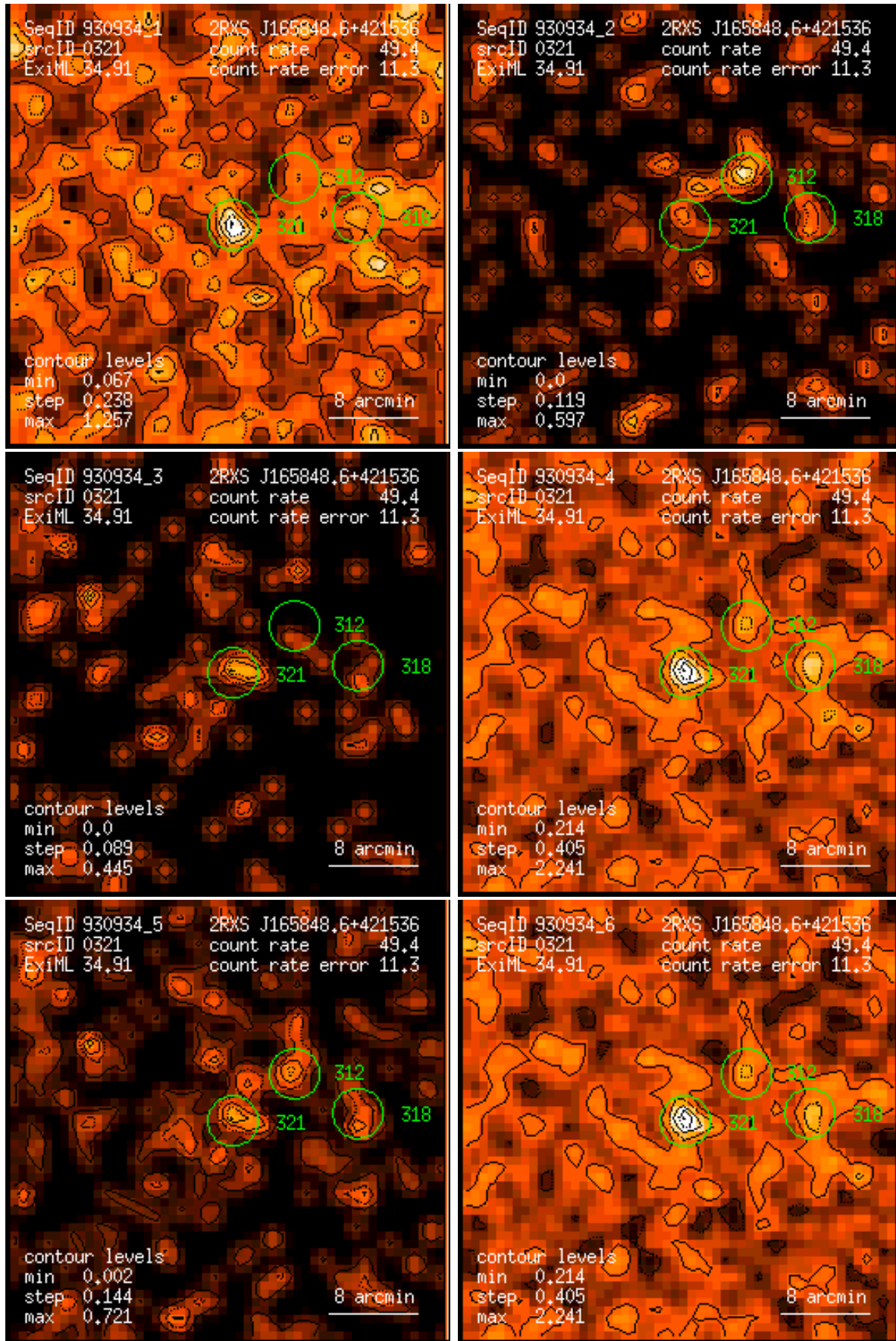
Figure 321: RASS 930934: detection 0321: band rate images, Gaussian filter: (1) PSPC channels 11 – 41, (2) 52 – 90, (3) 91 – 201, (4) 11 – 235, (5) 52 – 201, (6) 11 – 201. Broad band rates in counts/ks. Band rate contour levels in counts/ks/arcmin 2 .
