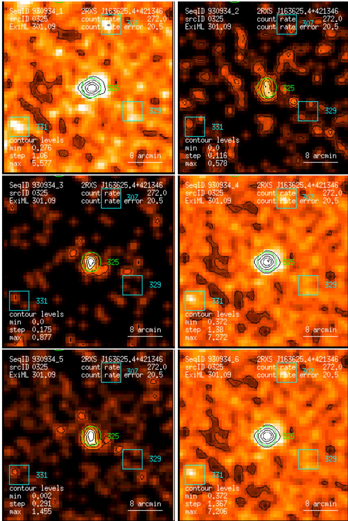
Figure 325: RASS 930934: detection 0325: band rate images, Gaussian filter: (1) PSPC channels 11 – 41, (2) 52 – 90, (3) 91 – 201, (4) 11 – 235, (5) 52 – 201, (6) 11 – 201. Broad band rates in counts/ks. Band rate contour levels in counts/ks/arcmin 2 .
