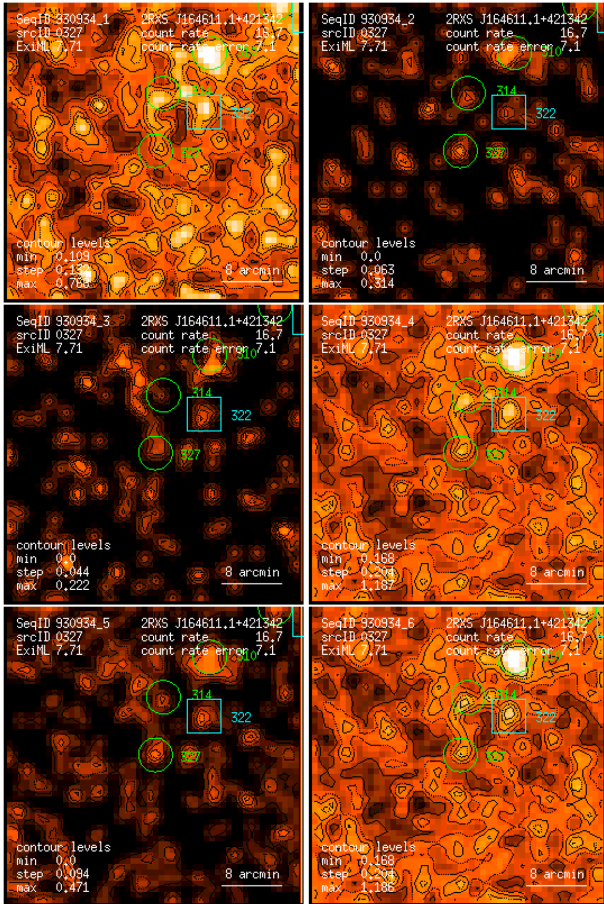
Figure 327: RASS 930934: detection 0327: band rate images, Gaussian filter: (1) PSPC channels 11 – 41, (2) 52 – 90, (3) 91 – 201, (4) 11 – 235, (5) 52 – 201, (6) 11 – 201. Broad band rates in counts/ks. Band rate contour levels in counts/ks/arcmin 2 .
