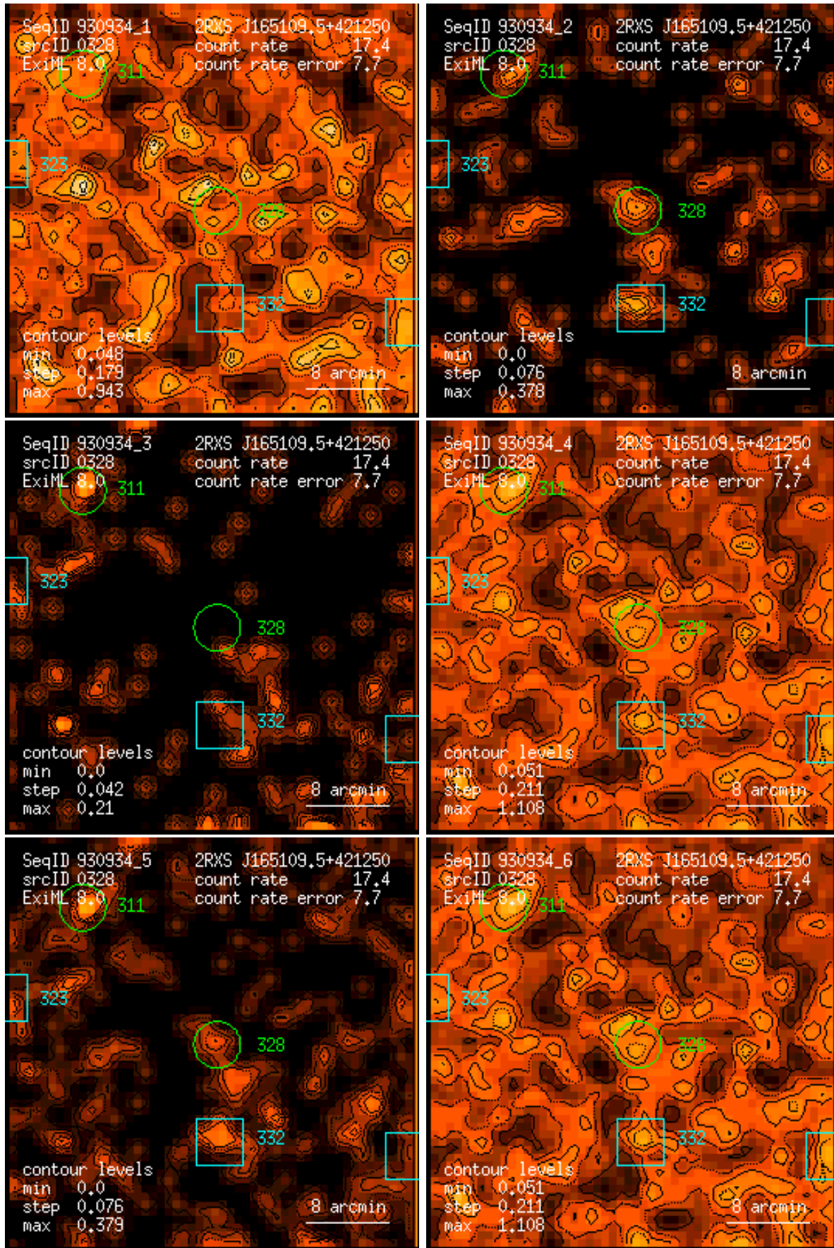
Figure 328: RASS 930934: detection 0328: band rate images, Gaussian filter: (1) PSPC channels 11 – 41, (2) 52 – 90, (3) 91 – 201, (4) 11 – 235, (5) 52 – 201, (6) 11 – 201. Broad band rates in counts/ks. Band rate contour levels in counts/ks/arcmin 2 .
