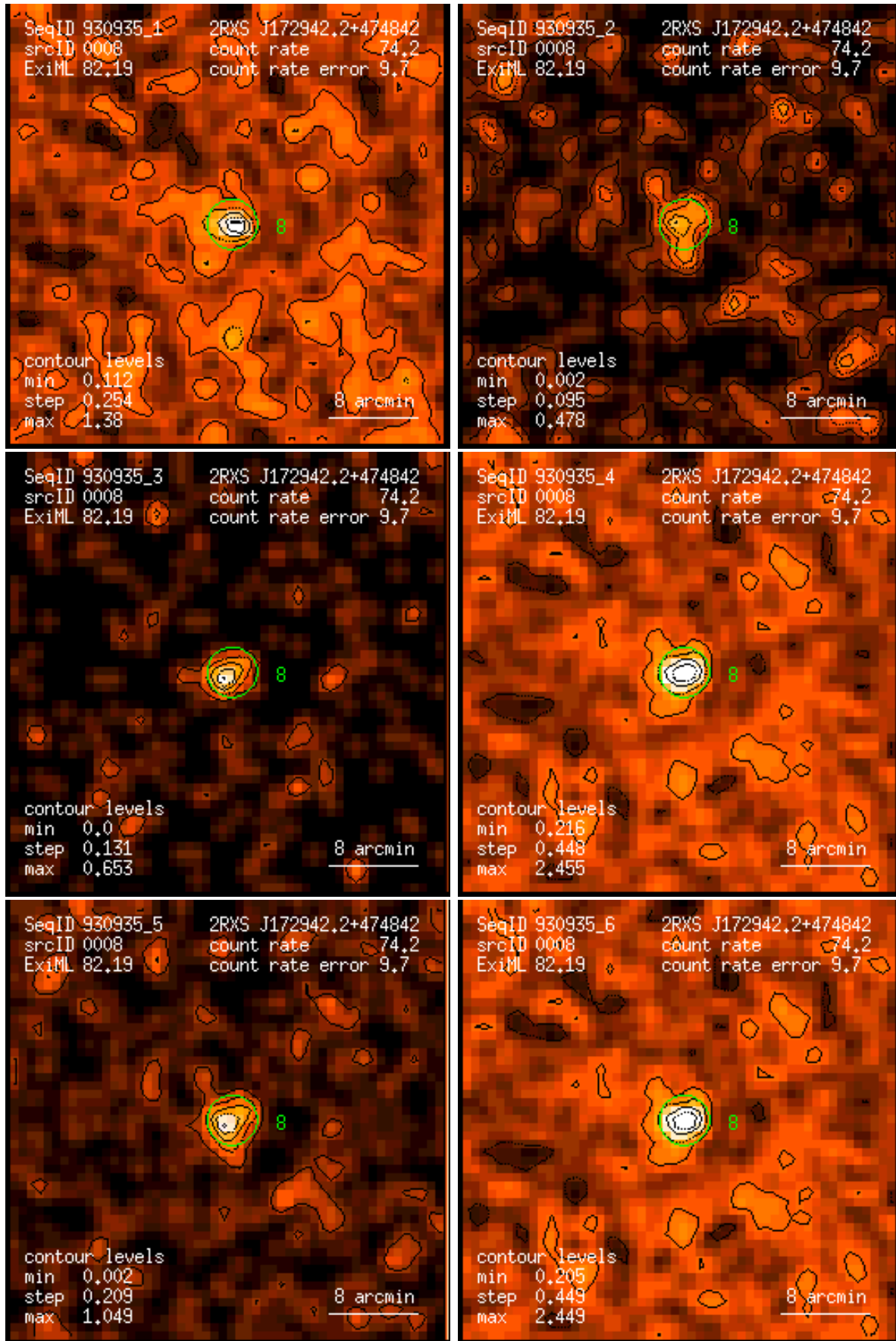
Figure 8: RASS 930935: detection 0008: band rate images, Gaussian filter: (1) PSPC channels 11 – 41, (2) 52 – 90, (3) 91 – 201, (4) 11 – 235, (5) 52 – 201, (6) 11 – 201. Broad band rates in counts/ks. Band rate contour levels in counts/ks/arcmin 2 .
