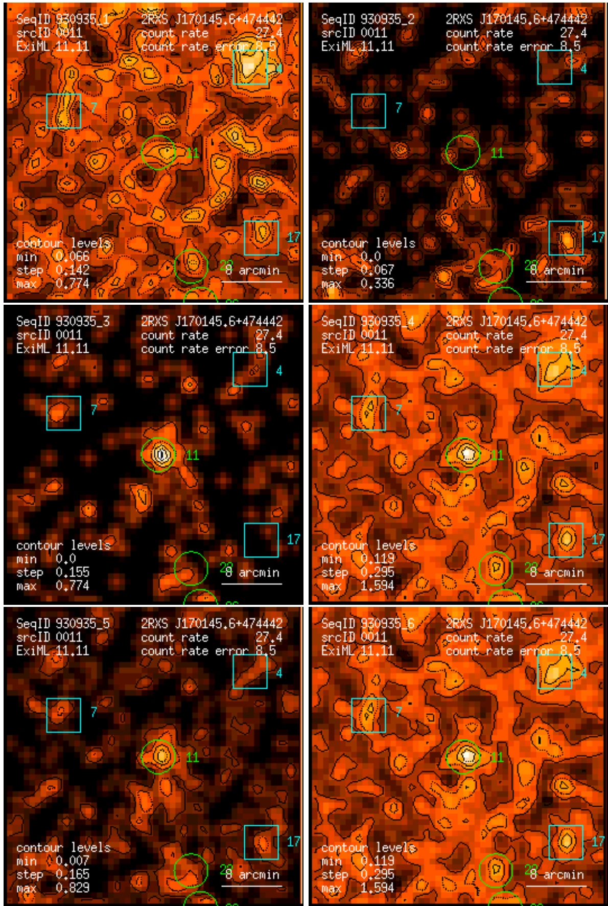
Figure 11: RASS 930935: detection 0011: band rate images, Gaussian filter: (1) PSPC channels 11 – 41, (2) 52 – 90, (3) 91 – 201, (4) 11 – 235, (5) 52 – 201, (6) 11 – 201. Broad band rates in counts/ks. Band rate contour levels in counts/ks/arcmin 2 .
