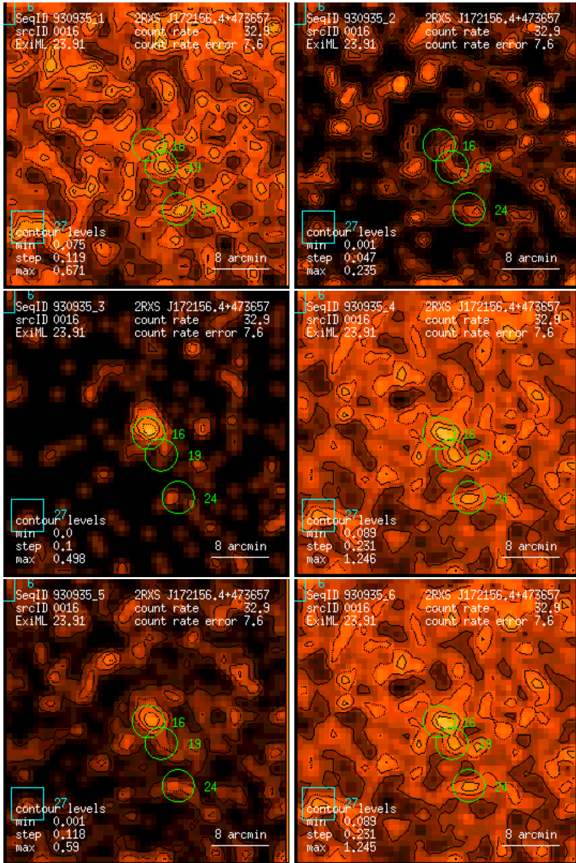
Figure 16: RASS 930935: detection 0016: band rate images, Gaussian filter: (1) PSPC channels 11 – 41, (2) 52 – 90, (3) 91 – 201, (4) 11 – 235, (5) 52 – 201, (6) 11 – 201. Broad band rates in counts/ks. Band rate contour levels in counts/ks/arcmin 2 .
