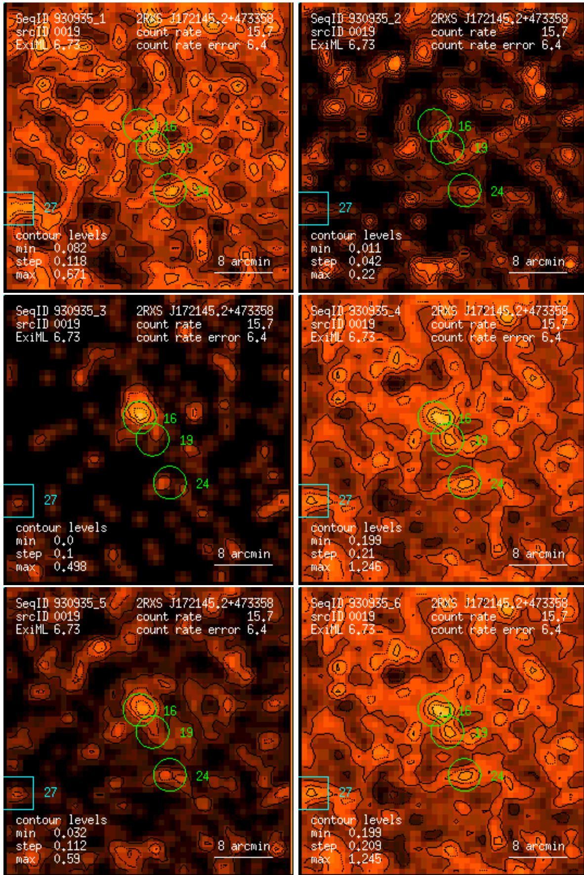
Figure 19: RASS 930935: detection 0019: band rate images, Gaussian filter: (1) PSPC channels 11 – 41, (2) 52 – 90, (3) 91 – 201, (4) 11 – 235, (5) 52 – 201, (6) 11 – 201. Broad band rates in counts/ks. Band rate contour levels in counts/ks/arcmin 2 .
