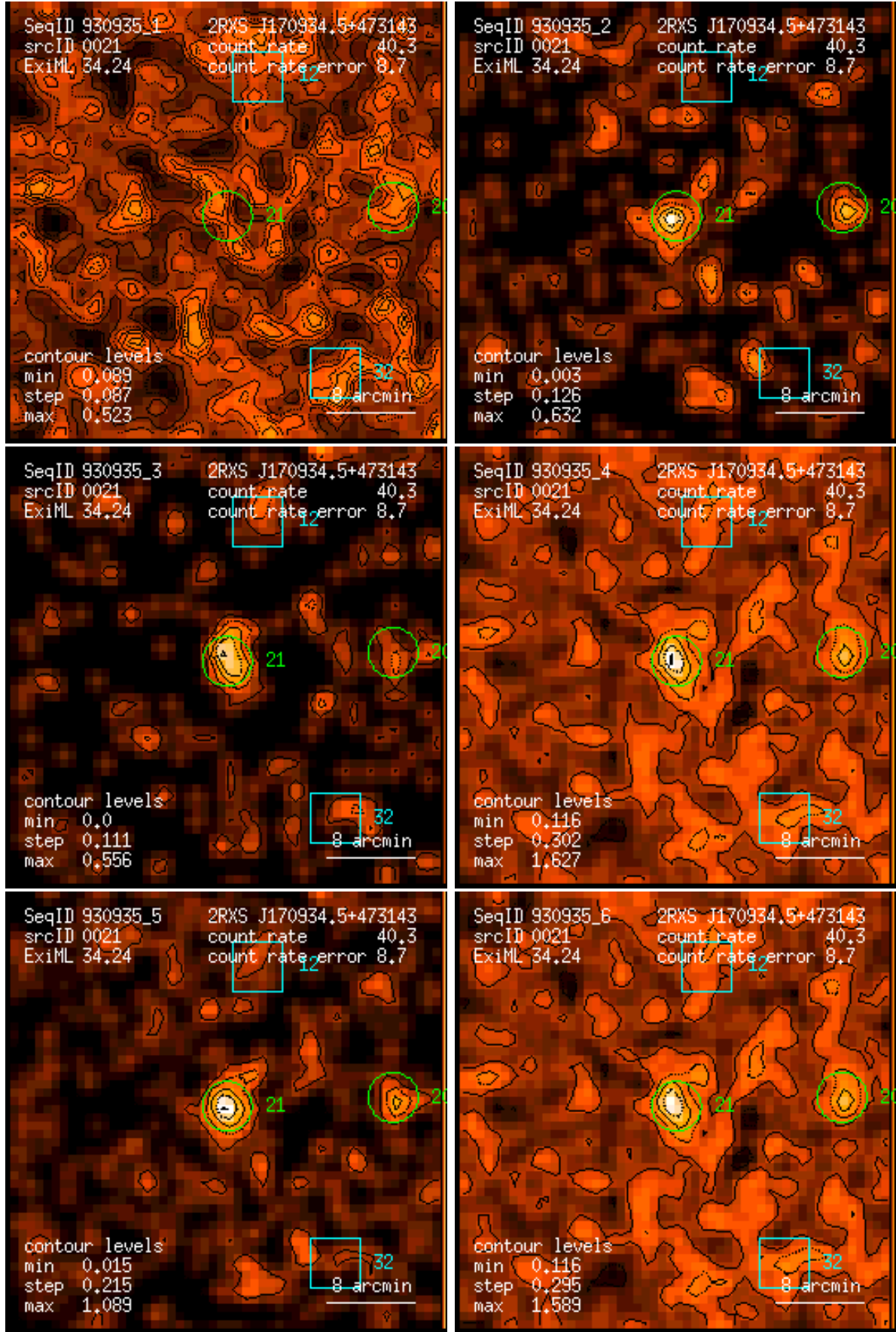
Figure 21: RASS 930935: detection 0021: band rate images, Gaussian filter: (1) PSPC channels 11 – 41, (2) 52 – 90, (3) 91 – 201, (4) 11 – 235, (5) 52 – 201, (6) 11 – 201. Broad band rates in counts/ks. Band rate contour levels in counts/ks/arcmin 2 .
