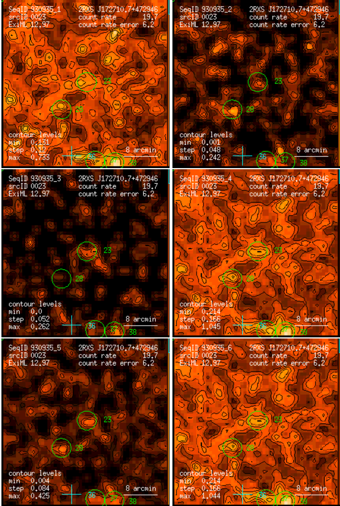
Figure 23: RASS 930935: detection 0023: band rate images, Gaussian filter: (1) PSPC channels 11 – 41, (2) 52 – 90, (3) 91 – 201, (4) 11 – 235, (5) 52 – 201, (6) 11 – 201. Broad band rates in counts/ks. Band rate contour levels in counts/ks/arcmin 2 .
