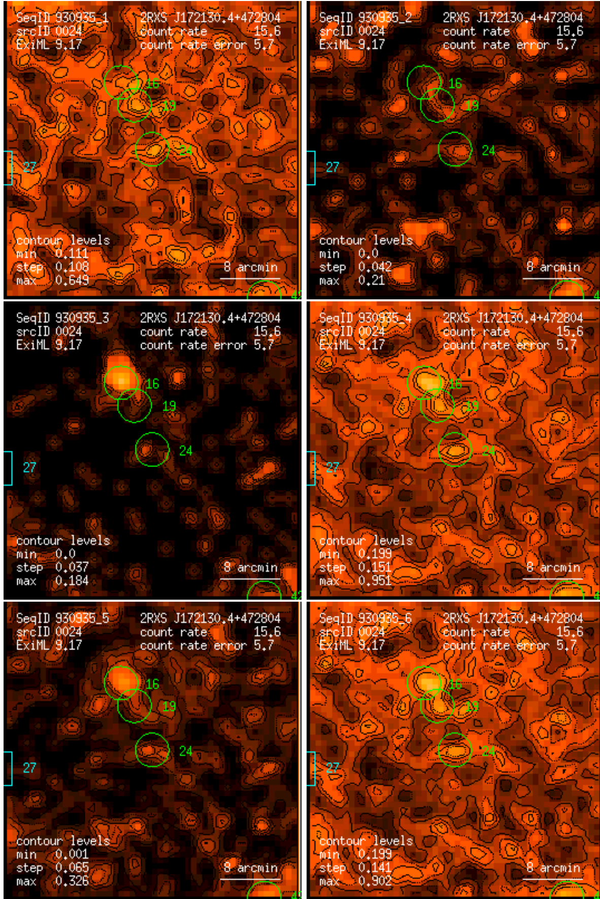
Figure 24: RASS 930935: detection 0024: band rate images, Gaussian filter: (1) PSPC channels 11 – 41, (2) 52 – 90, (3) 91 – 201, (4) 11 – 235, (5) 52 – 201, (6) 11 – 201. Broad band rates in counts/ks. Band rate contour levels in counts/ks/arcmin 2 .
