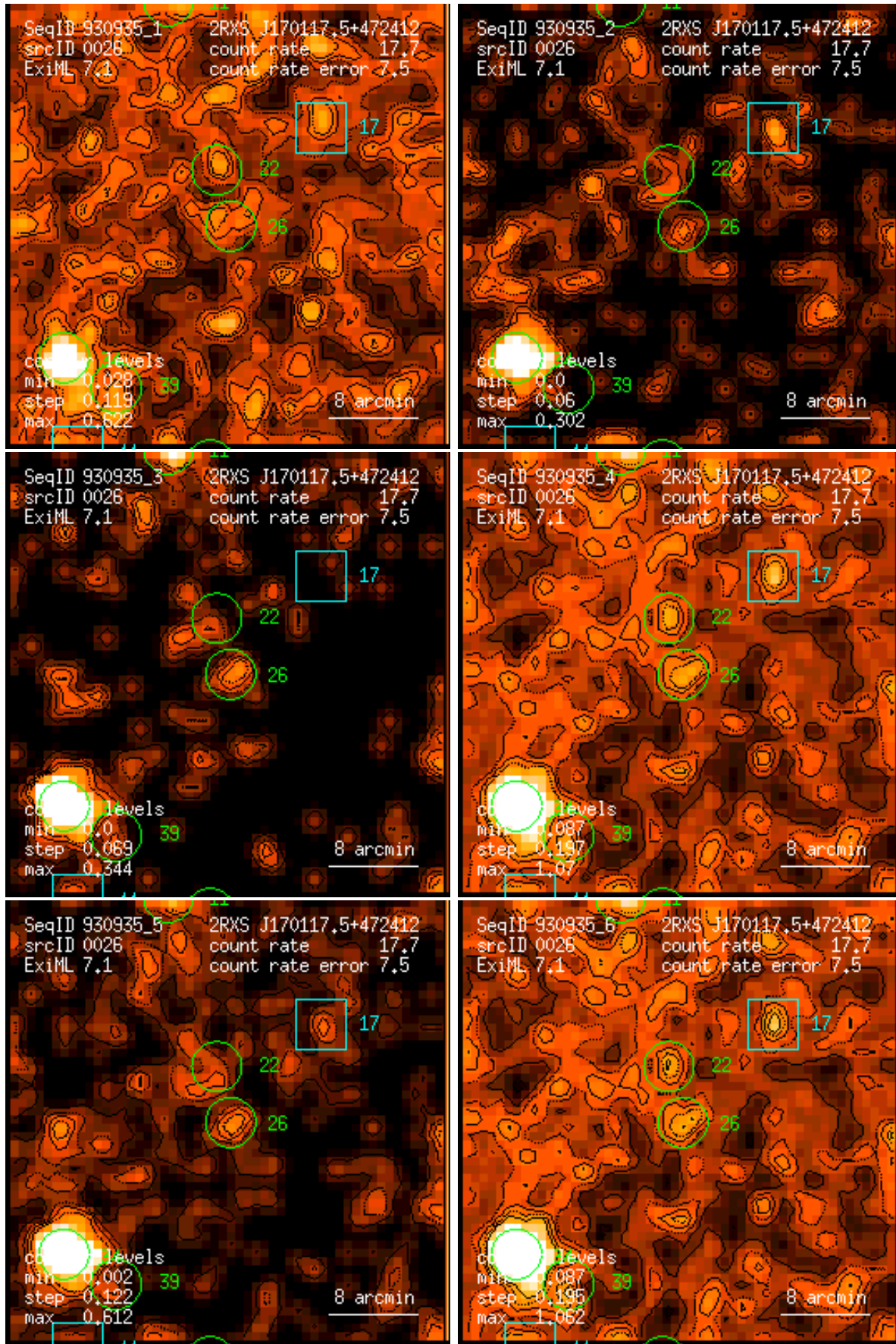
Figure 26: RASS 930935: detection 0026: band rate images, Gaussian filter: (1) PSPC channels 11 – 41, (2) 52 – 90, (3) 91 – 201, (4) 11 – 235, (5) 52 – 201, (6) 11 – 201. Broad band rates in counts/ks. Band rate contour levels in counts/ks/arcmin 2 .
