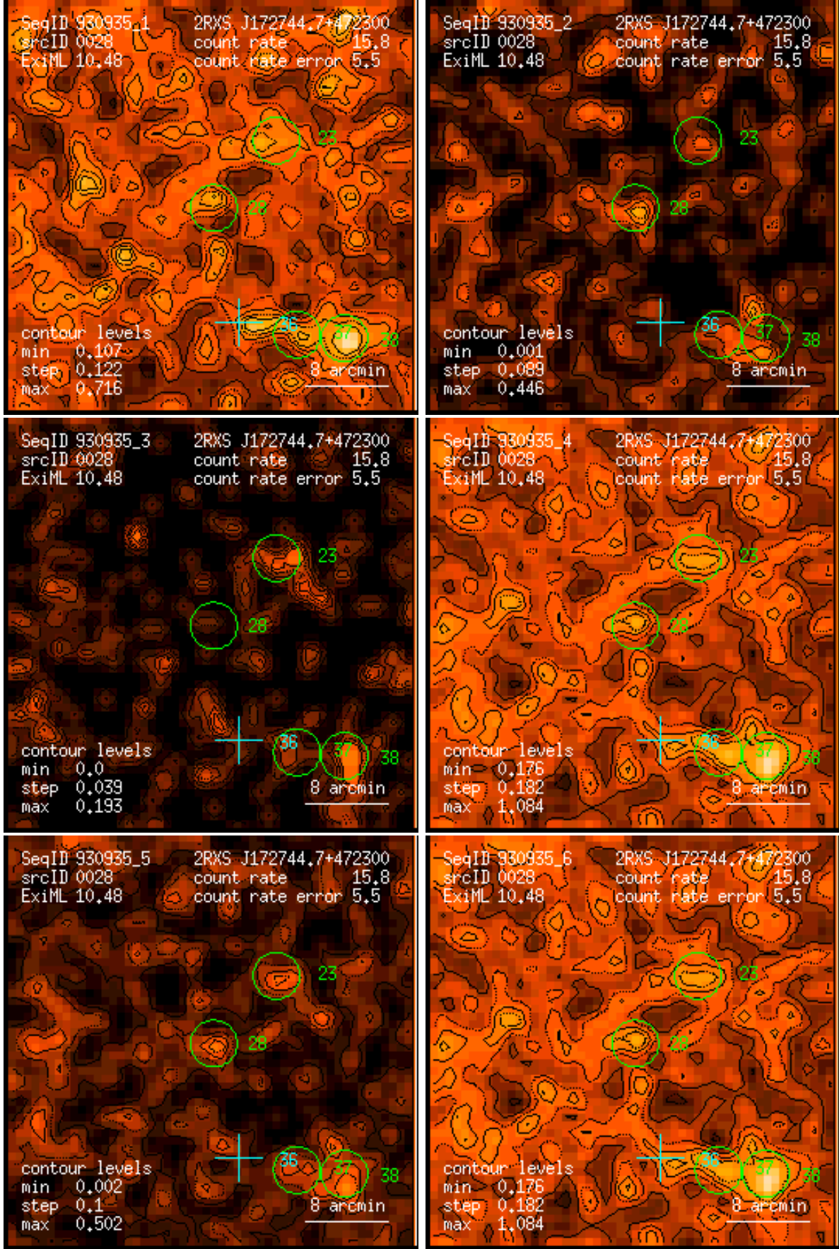
Figure 28: RASS 930935: detection 0028: band rate images, Gaussian filter: (1) PSPC channels 11 – 41, (2) 52 – 90, (3) 91 – 201, (4) 11 – 235, (5) 52 – 201, (6) 11 – 201. Broad band rates in counts/ks. Band rate contour levels in counts/ks/arcmin 2 .
