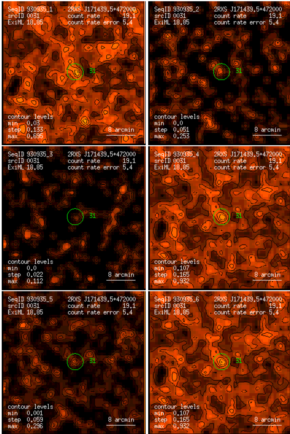
Figure 31: RASS 930935: detection 0031: band rate images, Gaussian filter: (1) PSPC channels 11 – 41, (2) 52 – 90, (3) 91 – 201, (4) 11 – 235, (5) 52 – 201, (6) 11 – 201. Broad band rates in counts/ks. Band rate contour levels in counts/ks/arcmin 2 .
