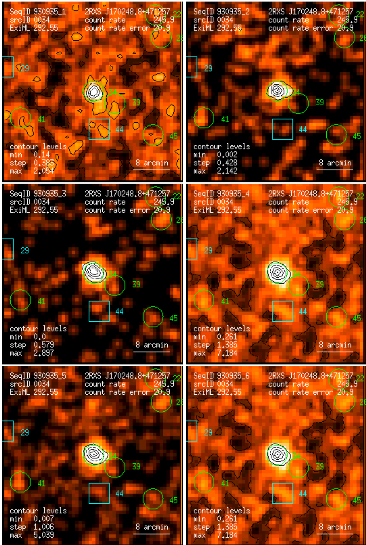
Figure 34: RASS 930935: detection 0034: band rate images, Gaussian filter: (1) PSPC channels 11 – 41, (2) 52 – 90, (3) 91 – 201, (4) 11 – 235, (5) 52 – 201, (6) 11 – 201. Broad band rates in counts/ks. Band rate contour levels in counts/ks/arcmin 2 .
