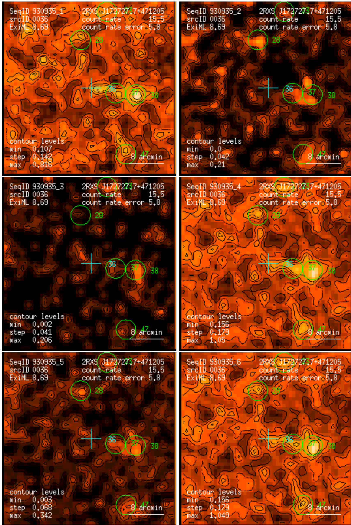
Figure 36: RASS 930935: detection 0036: band rate images, Gaussian filter: (1) PSPC channels 11 – 41, (2) 52 – 90, (3) 91 – 201, (4) 11 – 235, (5) 52 – 201, (6) 11 – 201. Broad band rates in counts/ks. Band rate contour levels in counts/ks/arcmin 2 .
