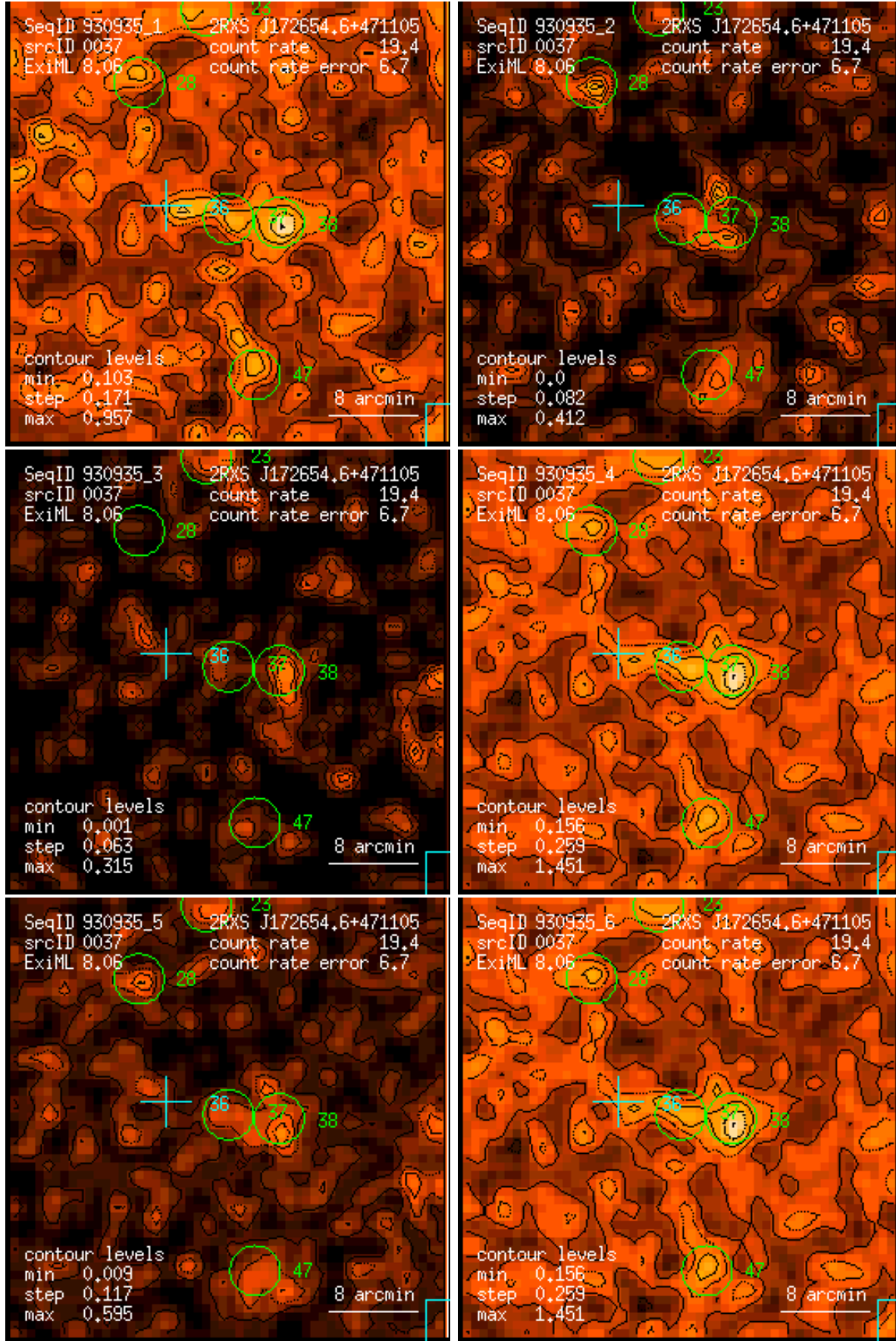
Figure 37: RASS 930935: detection 0037: band rate images, Gaussian filter: (1) PSPC channels 11 – 41, (2) 52 – 90, (3) 91 – 201, (4) 11 – 235, (5) 52 – 201, (6) 11 – 201. Broad band rates in counts/ks. Band rate contour levels in counts/ks/arcmin 2 .
